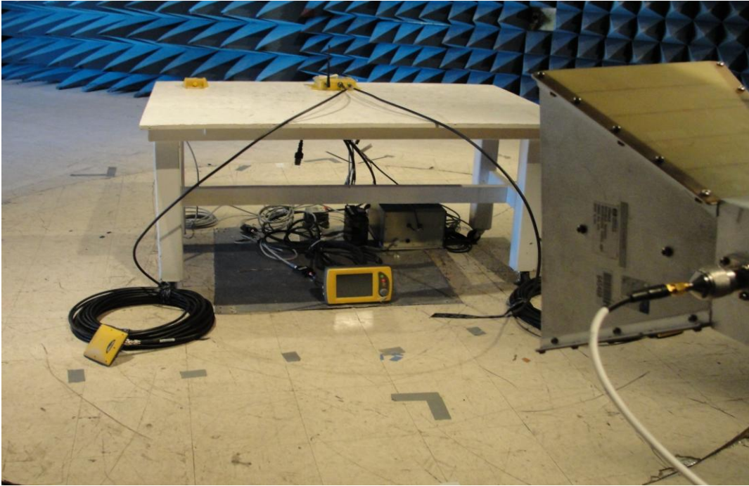
Figure 7: Radiated Test Set Up (1GHz – 18GHz) Horn Antenna Horizontal
