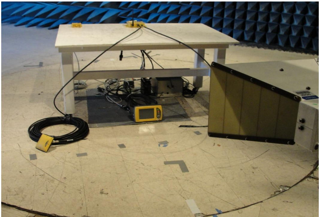
Figure 8: Radiated Test Set Up (1GHz – 18GHz) Horn Antenna Vertical
