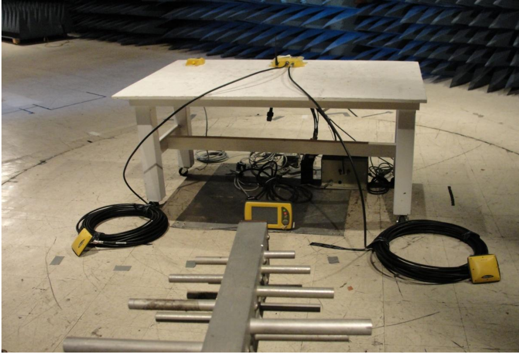
Figure 5: Radiated Test Set Up (200MHz – 1GHz) Log-Periodic Antenna Horizontal
