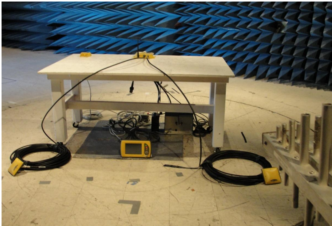
Figure 6: Radiated Test Set Up (200MHz – 1GHz) Log-Periodic Antenna Vertical
