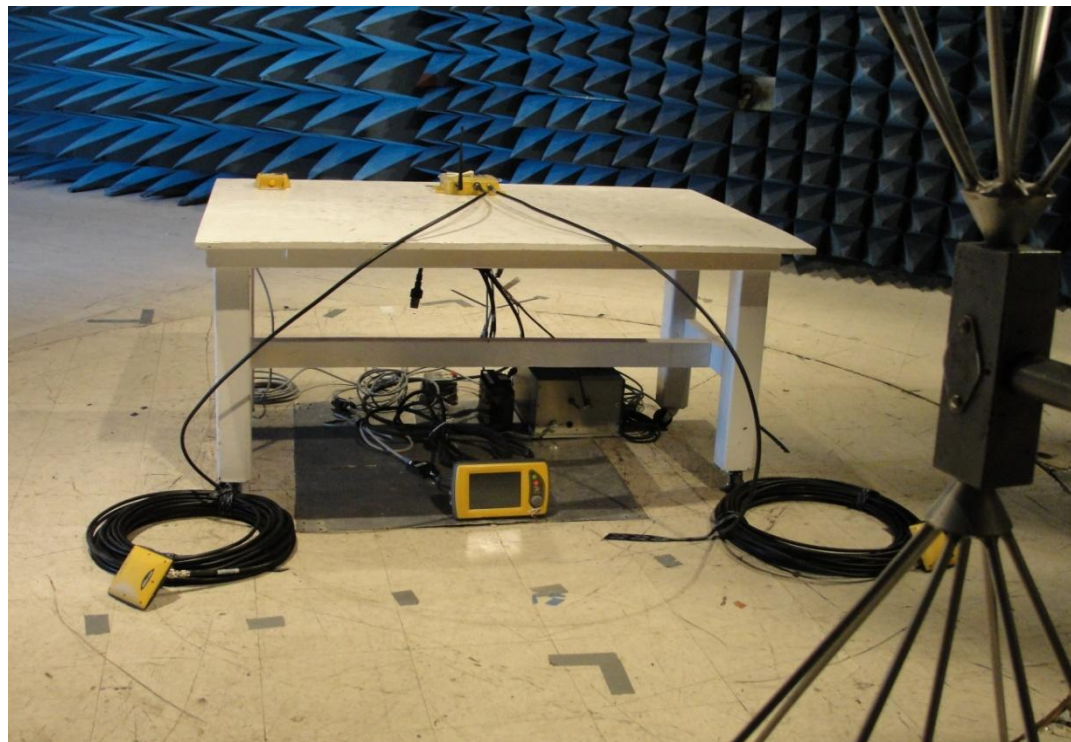
Figure 4: Radiated Test Set Up (30MHz – 200MHz) Biconical Antenna Vertical
