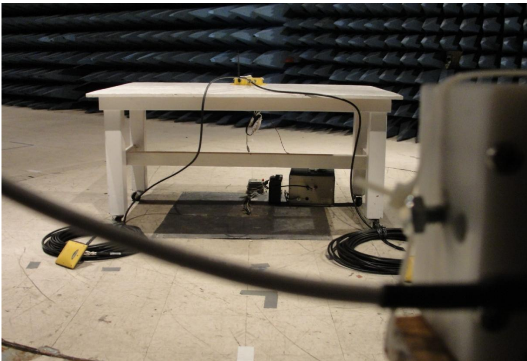
Figure 2: Radiated Test Set Up (18GHz – 24GHz) SHF-EHF Horn Antenna
