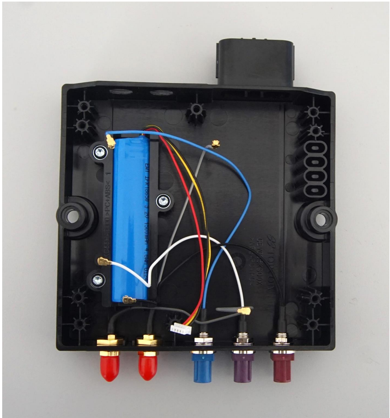
Internal battery
