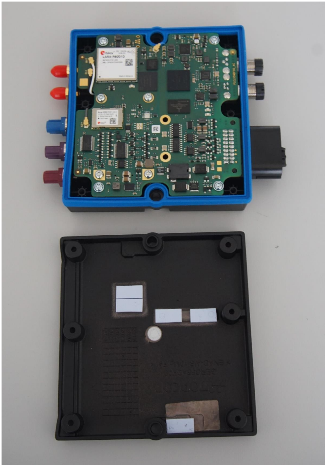
Open casing
