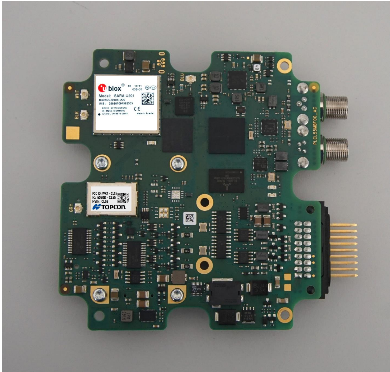
u-blox AG type SARA-U201 and Topcon Positioning Systems CL-55
