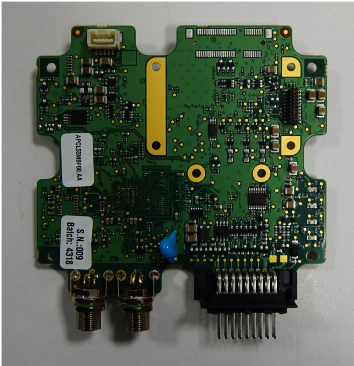
Bottom side without UHF radio embedded
