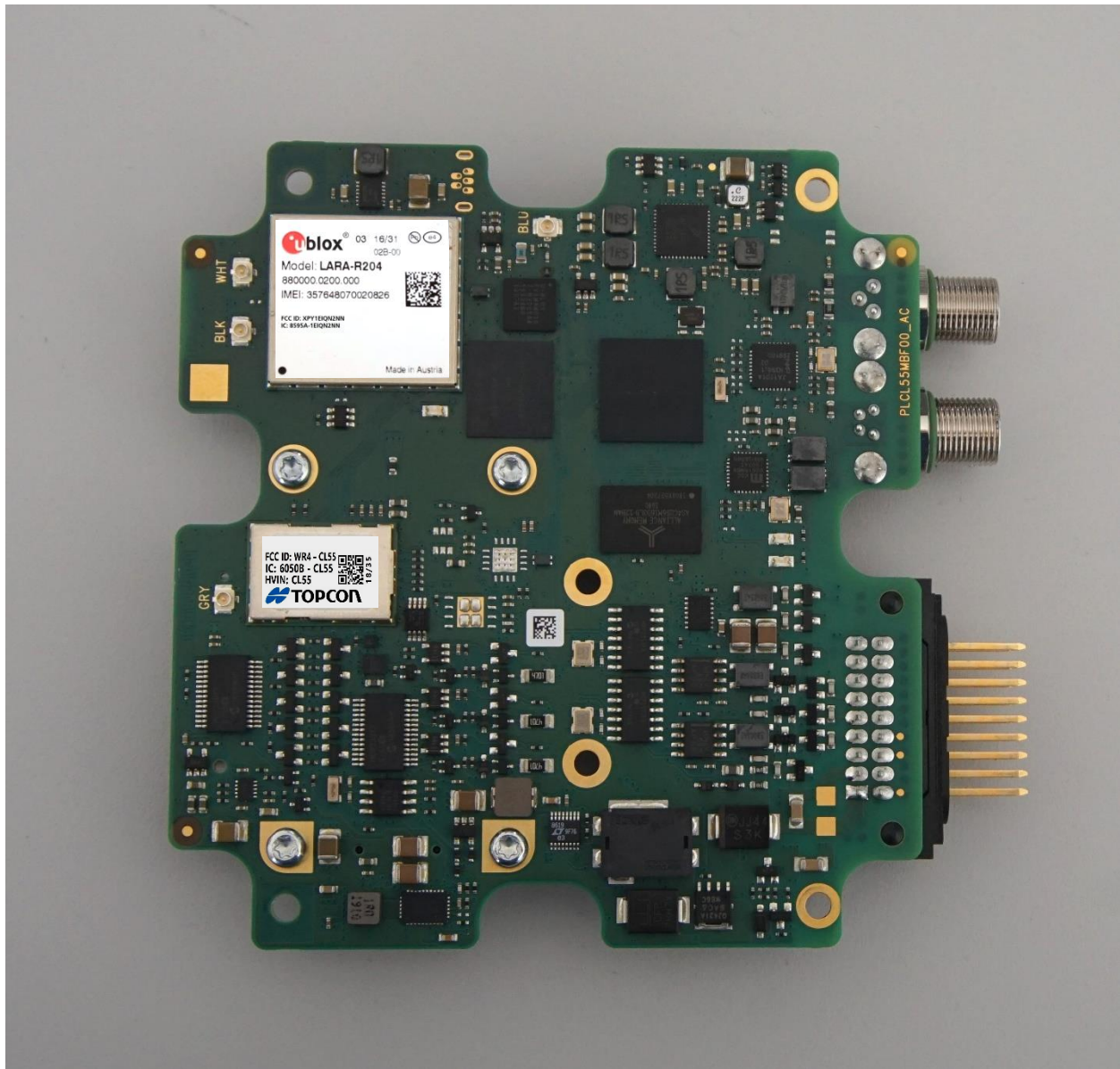
u-blox AG type LARA-R204 and Topcon Positioning Systems CL-55
