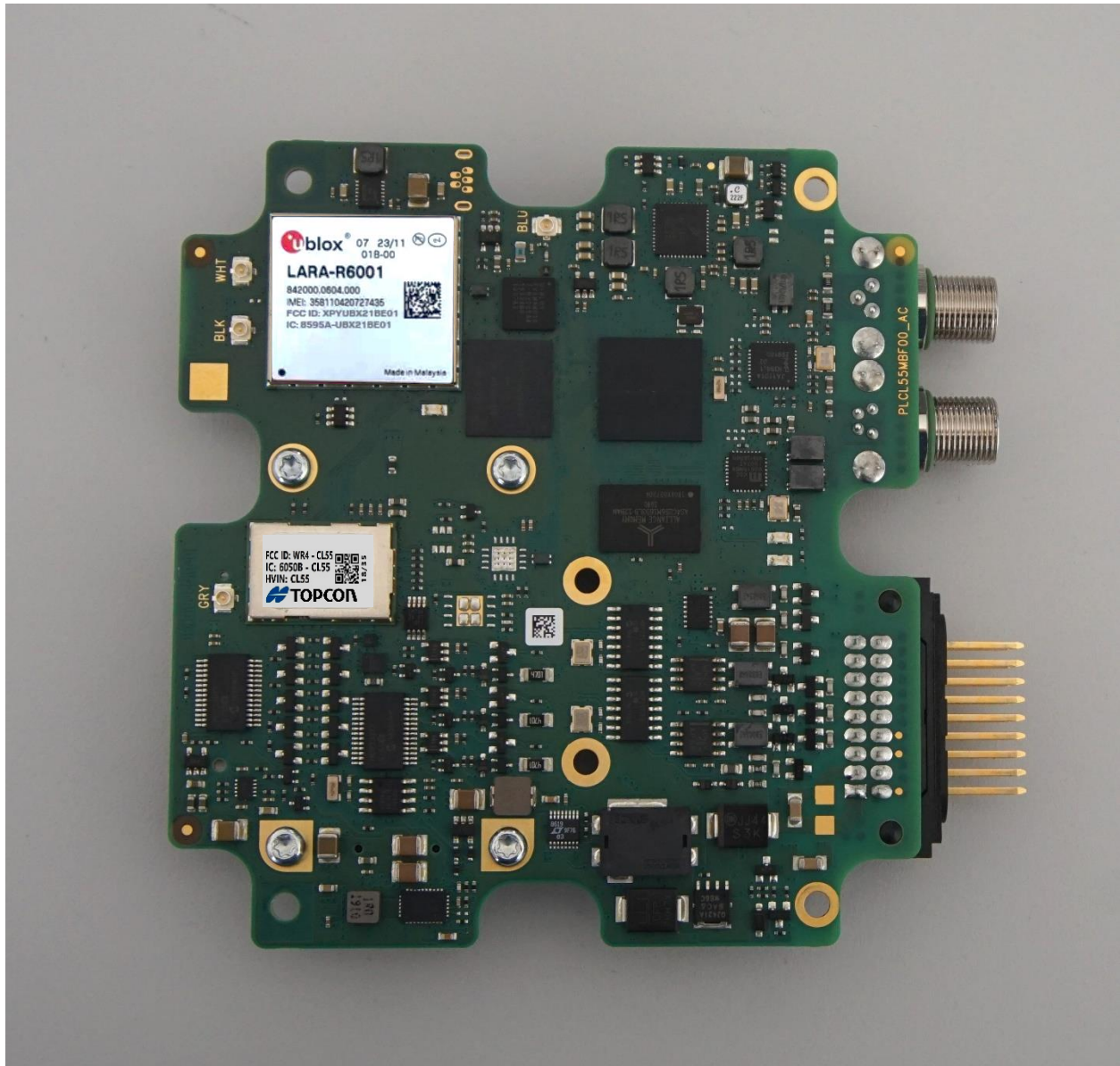
u-blox AG type LARA-R6001D and Topcon Positioning Systems CL-55
