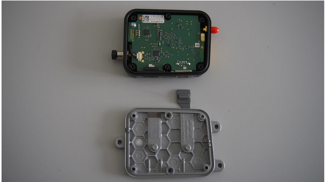
Open casing
