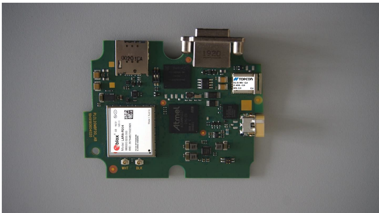
u-blox AG type LARA-R204 and Topcon Positioning Systems CL-20
