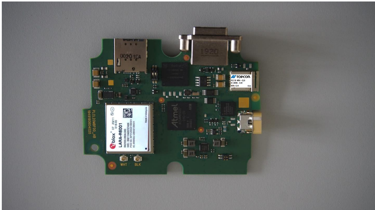
u-blox AG type LARA-R6001D and Topcon Positioning Systems CL-20
