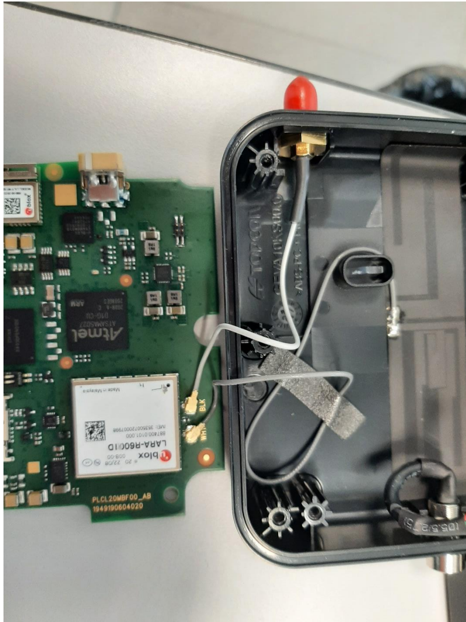
Tekfun FX-W06 LTE internal antenna plugged on internal case and connected to u-blox AG type LARA-R6001D
