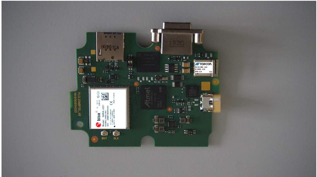
u-blox AG type SARA-U201 and Topcon Positioning Systems CL-20
