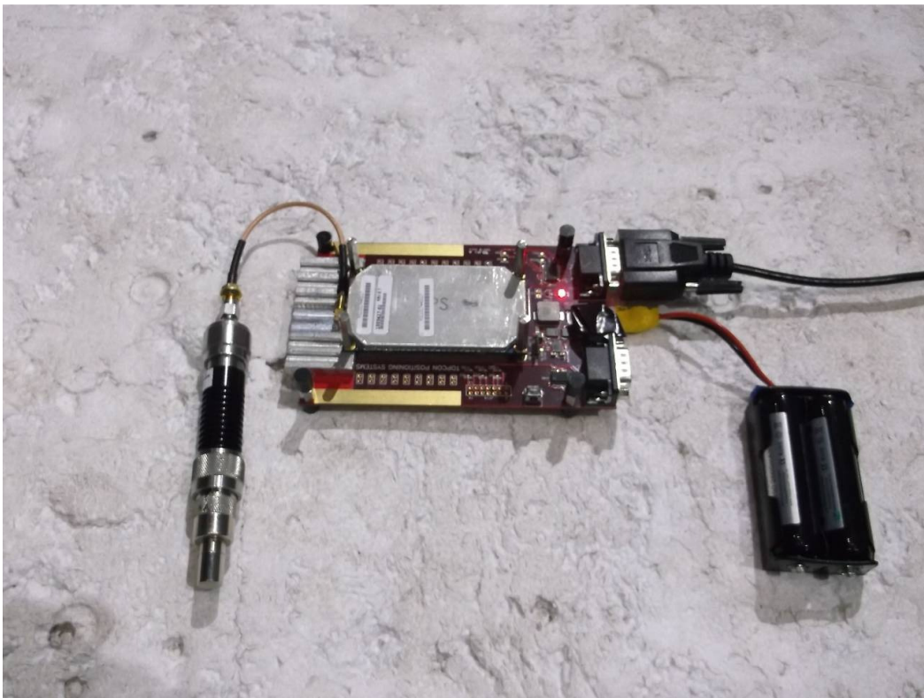
Radiated emissions - EUT Flat on the table
