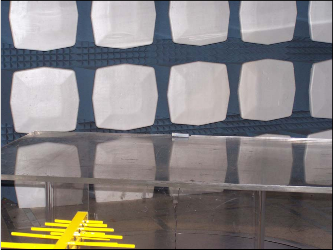
Photograph 2. Radiated Emissions, Test Setup
