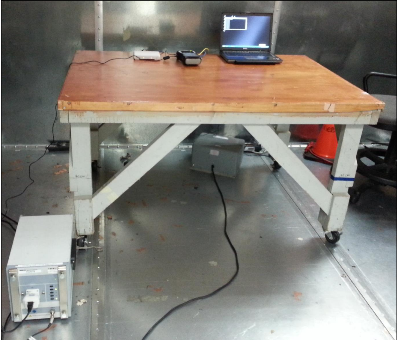
Photograph 1. Conducted Emissions, Test Setup
