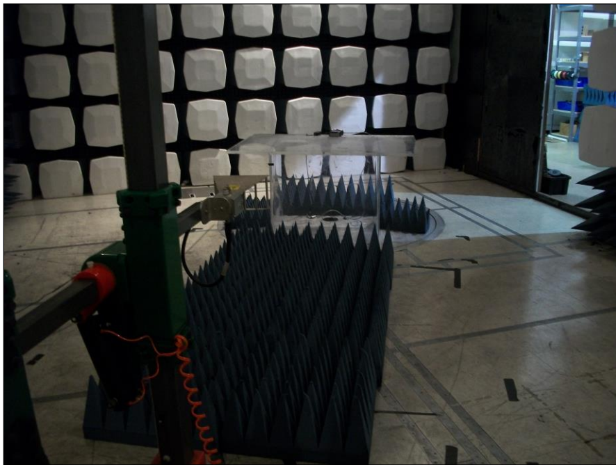
Photograph 3. Radiated Emissions, Test Setup, Above 1 GHz
