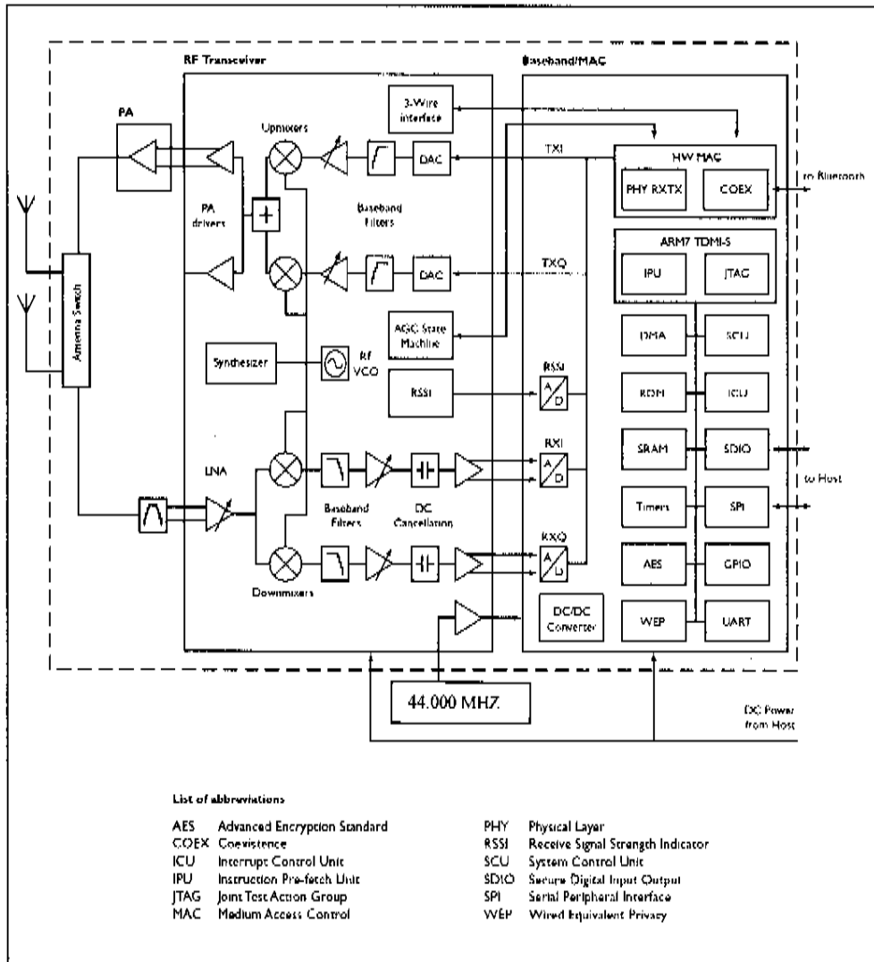
BGW200 functional block diagram
