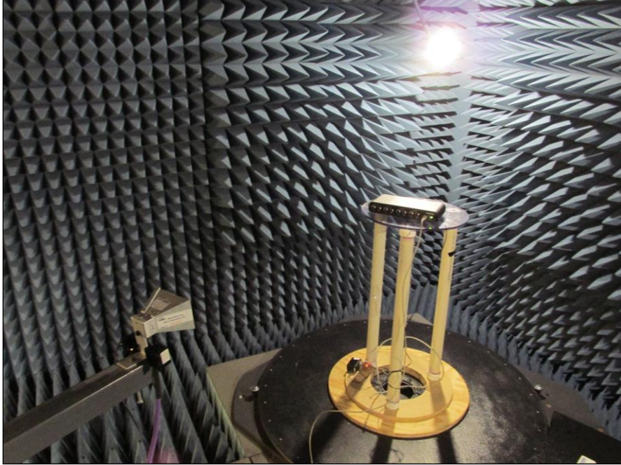
Photograph 7. Radiated Spurious Emissions, Test Setup, 18 GHz – 25 GHz
