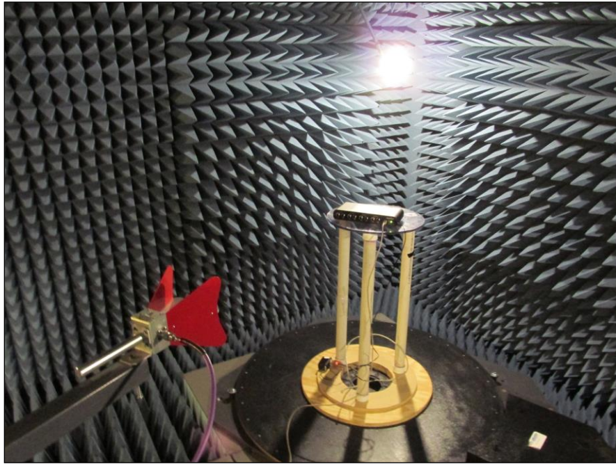
Photograph 5. Radiated Spurious Emissions, Test Setup, 1 GHz – 7 GHz
