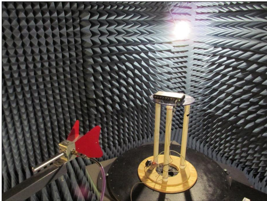
Photograph 6. Radiated Spurious Emissions, Test Setup, 7 GHz – 18 GHz
