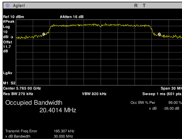
Plot 5. Occupied Bandwidth, 802.11n, Mid Channel
