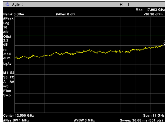
Plot 24. Radiated Spurious Emissions, 802.11a, Worst Case, 7 GHz – 18 GHz
