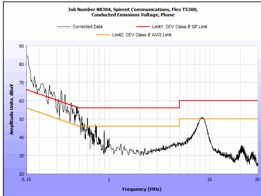
Plot 39. Conducted Emissions, Phase Line
