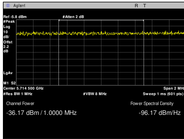
Plot 30. Radiated Band Edge, 802.11a, Low Channel, 5715 MHz Integration
