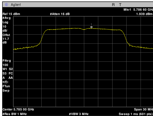
Plot 14. Maximum Power Spectral Density, 802.11a, Mid Channel
