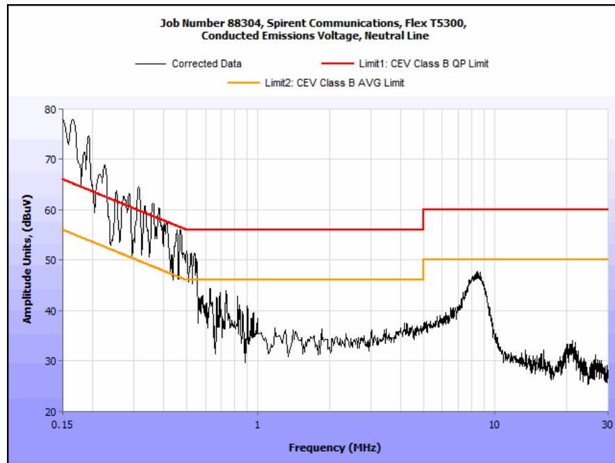
Plot 40. Conducted Emissions, Neutral Line
