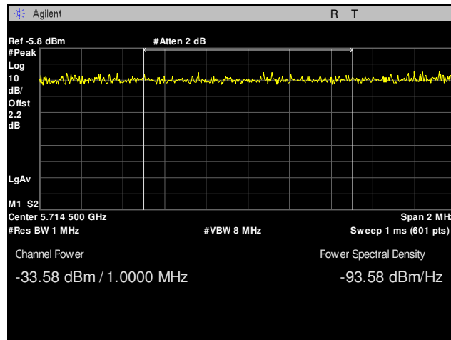
Plot 35. Radiated Band Edge, 802.11n, Low Channel, 5715 MHz Integration
