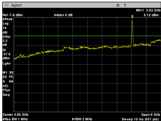
Plot 27. Radiated Spurious Emissions, 802.11n, High Channel, 1 GHz – 7 GHz
