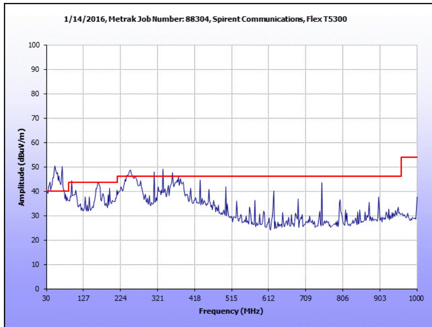
Plot 20. Radiated Spurious Emissions, 30 MHz – 1 GHz Radio OFF
