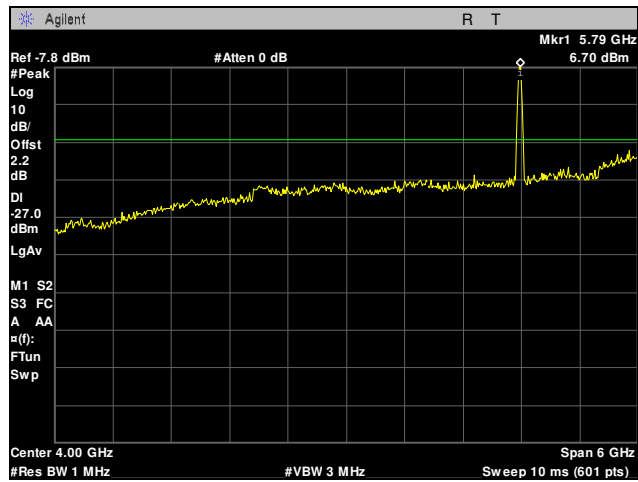
Plot 22. Radiated Spurious Emissions, 802.11a, Mid Channel, 1 GHz – 7 GHz
