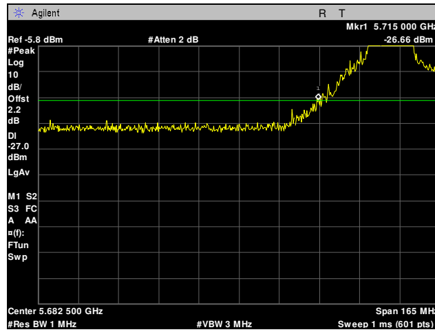
Plot 29. Radiated Band Edge, 802.11a, Low Channel
