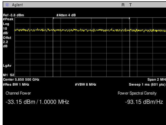
Plot 33. Radiated Band Edge, 802.11a, High Channel, 5850 MHz Integration
