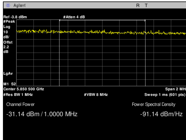
Plot 38. Radiated Band Edge, 802.11n, High Channel, 5850 MHz Integration
