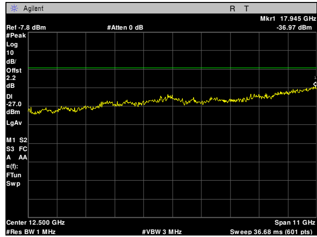
Plot 28. Radiated Spurious Emissions, 802.11n, Worst Case, 7 GHz – 18 GHz
