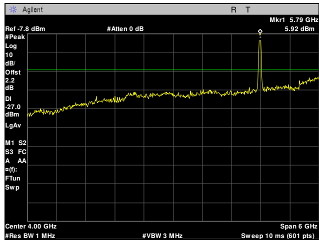
Plot 26. Radiated Spurious Emissions, 802.11n, Mid Channel, 1 GHz – 7 GHz
