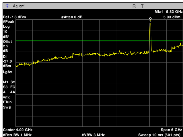
Plot 23. Radiated Spurious Emissions, 802.11a, High Channel, 1 GHz – 7 GHz
