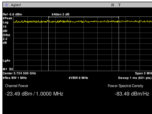
Plot 36. Radiated Band Edge, 802.11n, Low Channel, 5725 MHz Integration
