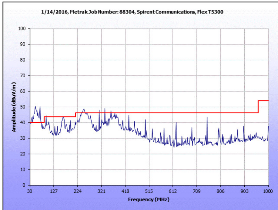
Plot 19. Radiated Spurious Emissions, 30 MHz – 1 GHz Radio On
