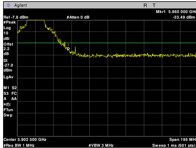
Plot 32. Radiated Band Edge, 802.11a, High Channel
