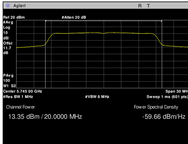
Plot 10. Maximum Conducted Output Power, 802.11n, Low Channel
