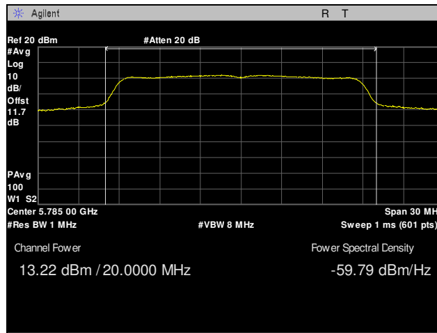
Plot 11. Maximum Conducted Output Power, 802.11n, Mid Channel
