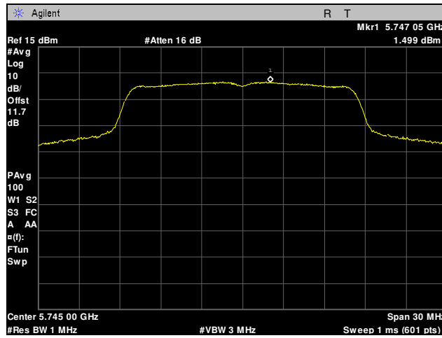
Plot 13. Maximum Power Spectral Density, 802.11a, Low Channel
