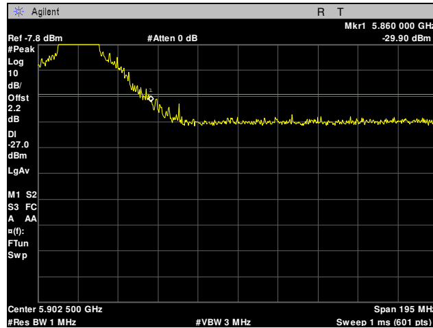
Plot 37. Radiated Band Edge, 802.11n, High Channel
