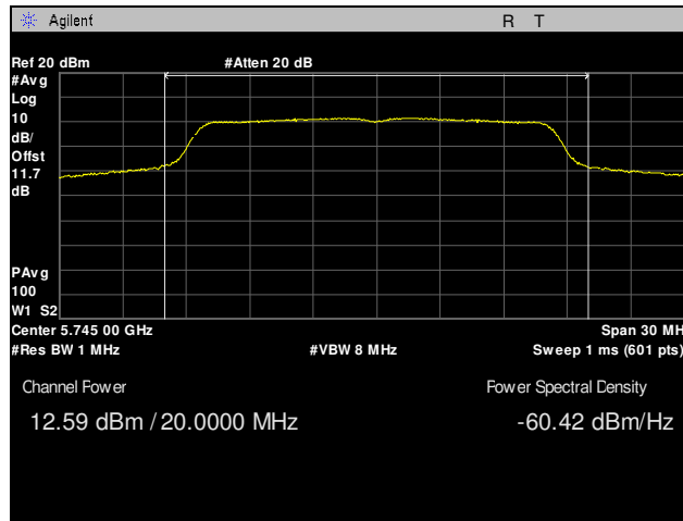
Plot 7. Maximum Conducted Output Power, 802.11a, Low Channel
