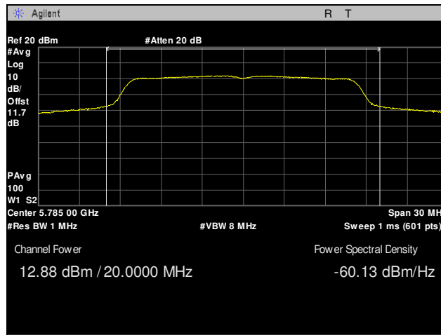
Plot 8. Maximum Conducted Output Power, 802.11a, Mid Channel
