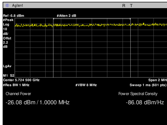
Plot 31. Radiated Band Edge, 802.11a, Low Channel, 5725 MHz Integration
