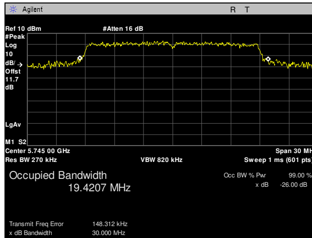
Plot 4. Occupied Bandwidth, 802.11n, Low Channel
