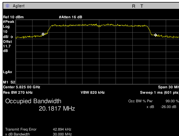
Plot 6. Occupied Bandwidth, 802.11n, High Channel
