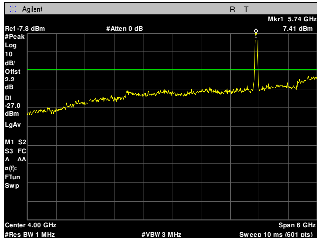
Plot 25. Radiated Spurious Emissions, 802.11n, Low Channel, 1 GHz – 7 GHz
