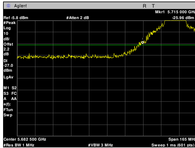
Plot 34. Radiated Band Edge, 802.11n, Low Channel
