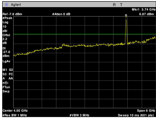
Plot 21. Radiated Spurious Emissions, 802.11a, Low Channel, 1 GHz – 7 GHz
