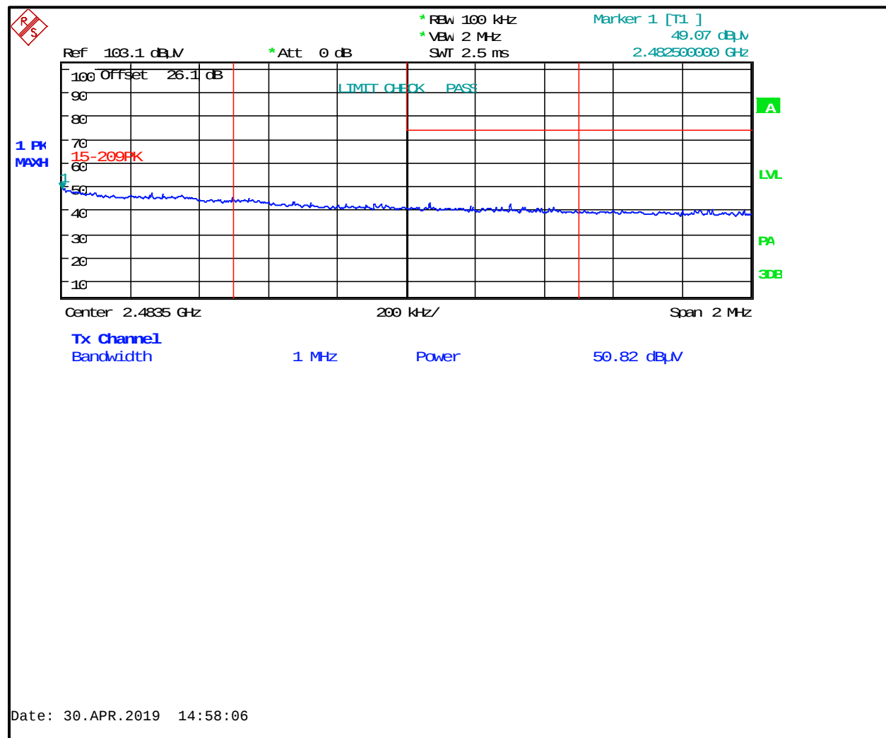
Plot 4-4: Integrated Upper Band Edge - Channel 26 (2480 MHz) Peak
