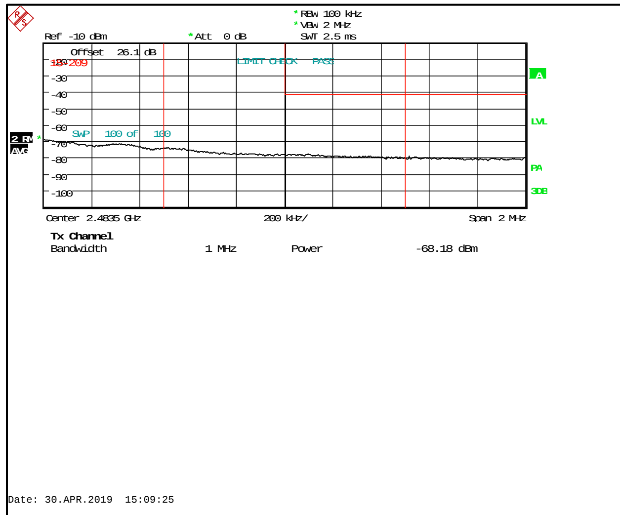
Plot 4-3: Integrated Upper Band Edge - Channel 26 (2480 MHz) RMS
