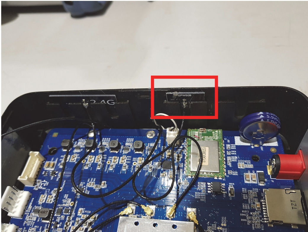
WLAN 5GHz_Antenna 3
