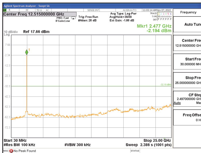
ANT2, 802.11ax_HE20_242T
