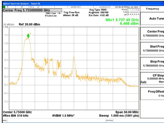
ANT1_802.11ax_HE40_26T_UNII 3
