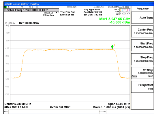
ANT1_802.11ax_HE40_484T_UNII 1
