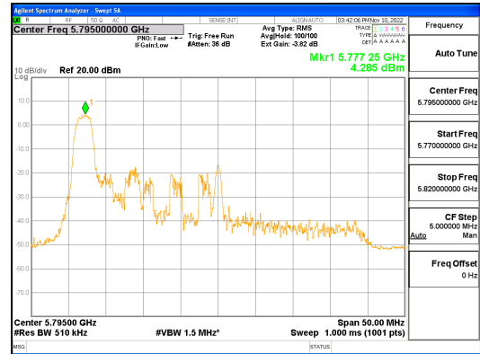
ANT1_802.11ax_HE40_26T_UNII 3
