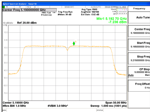
ANT1_802.11ac_VHT40_UNII 1
