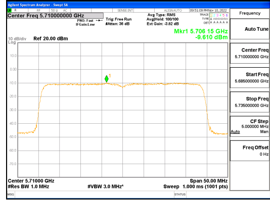
ANT1_802.11ax_HE40_484T_UNII 2C
