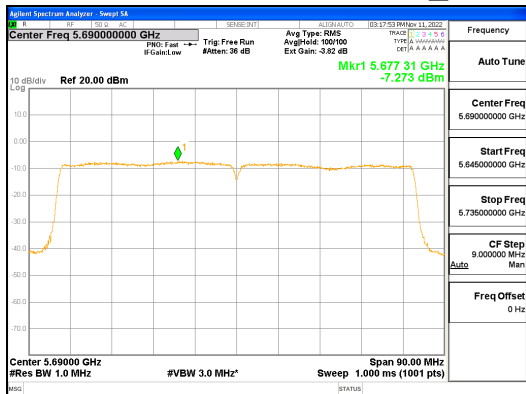
ANT1_802.11ac_VHT80_UNII 2C
