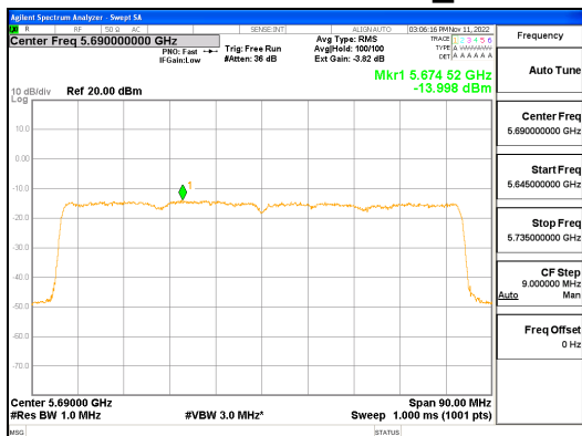
ANT1_802.11ax_HE80_996T_UNII 2C
