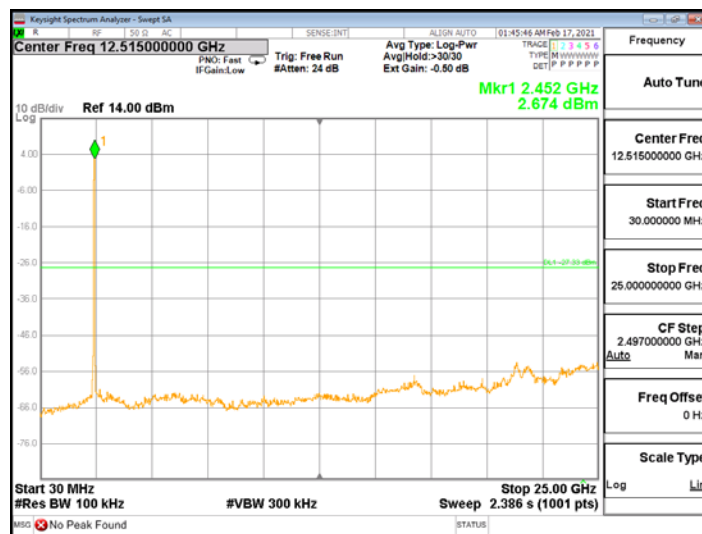
ANT3, 802.11n_HT40
