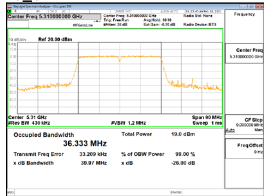
ANT1_802.11n_HT40_UNI 2A
