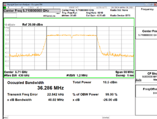
ANT1_802.11n_HT40_UNI 2C
