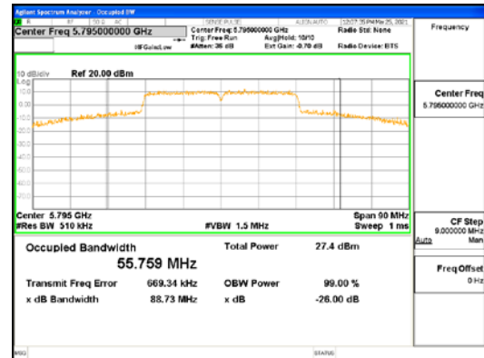
ANT4_802.11n_HT40_UNI1 3
