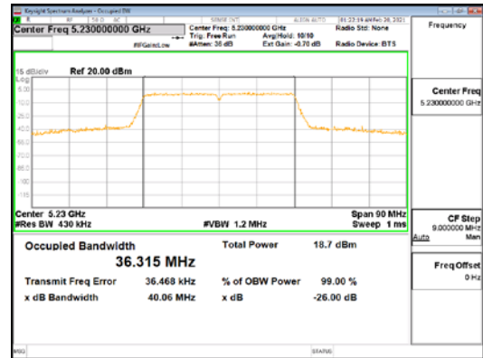
ANT1_802.11n_HT40_UNI 1
