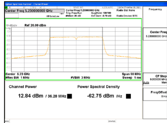
ANT4_802.11ac_VHT40_UNI I
