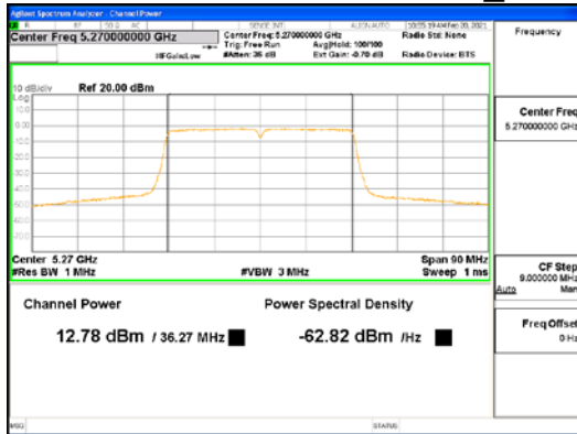
ANT4_802.11ac_VHT40_UNI I 2A
