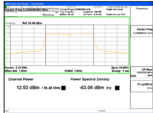
ANT4_802.11n_HT40_UNI I 1
