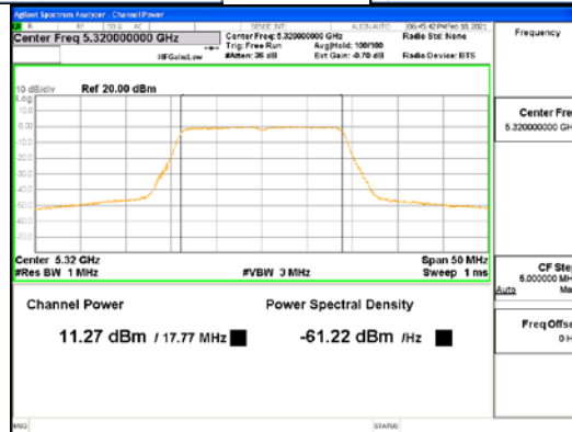
ANT2_802.11ac_VHT20_UNII 2A
