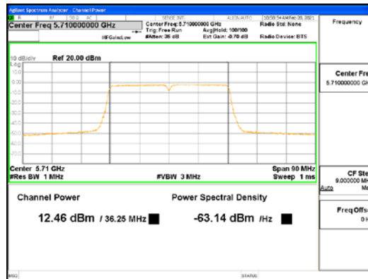
ANT4_802.11ac_VHT40_UNI I 2C
