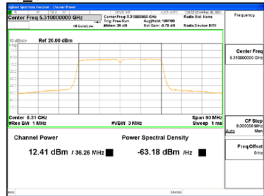
ANT4_802.11n_HT40_UNI I 2A
