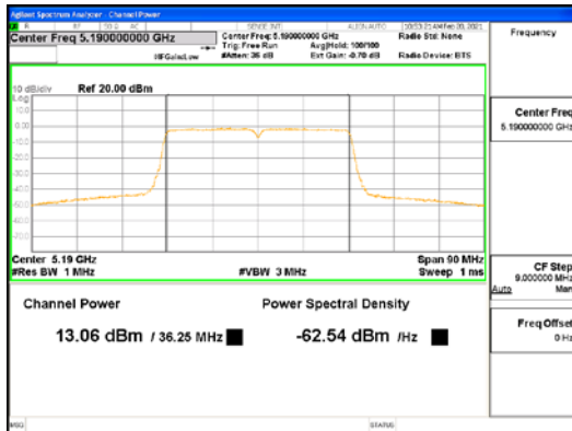
ANT4_802.11ac_VHT40_UNI I
