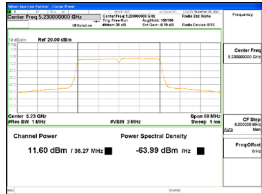
ANT2_802.11ac_VHT40_UNI I
