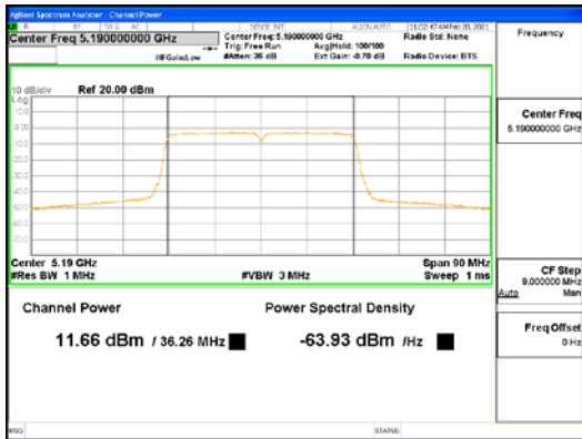
ANT2_802.11ac_VHT40_UNI I
