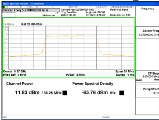
ANT2_802.11ac_VHT40_UNI I 2A
