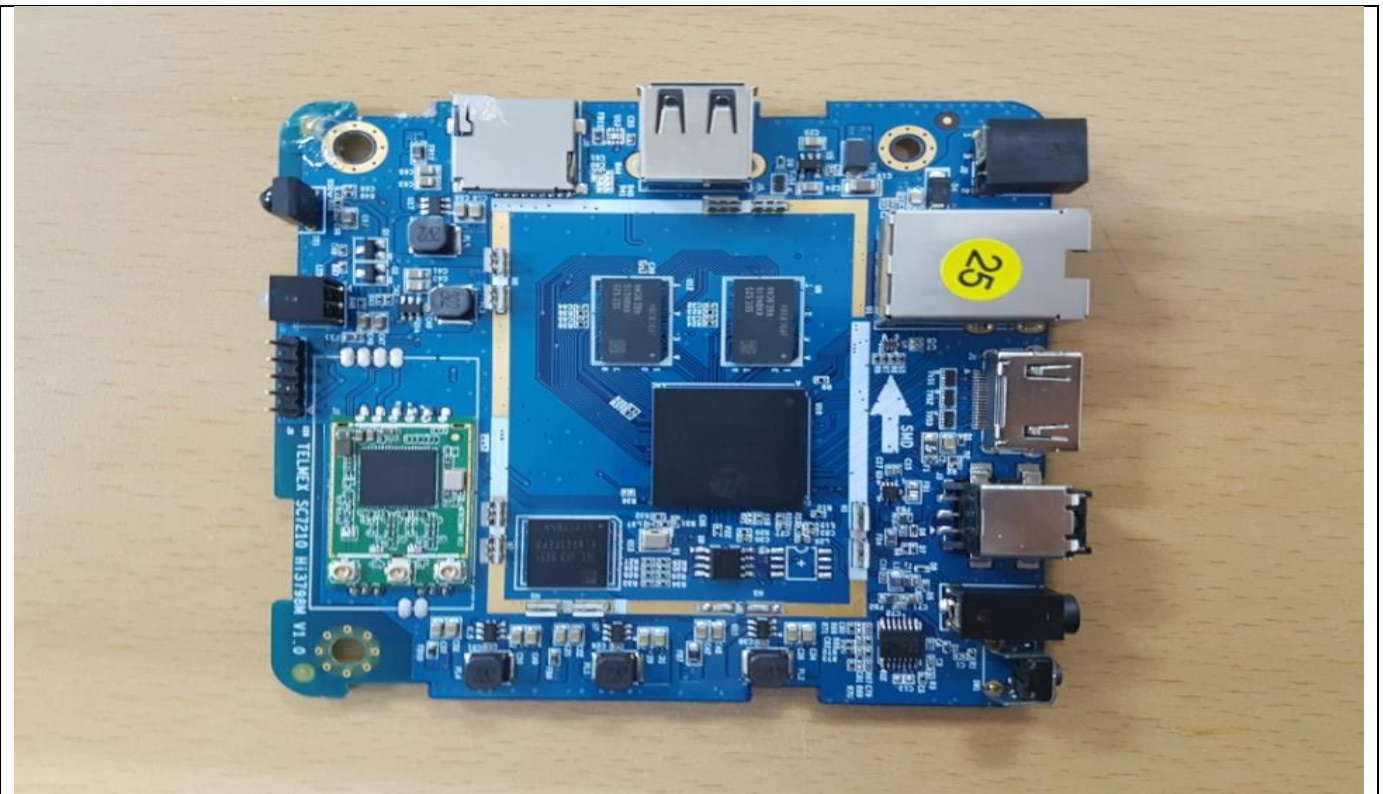
Board (Top)
