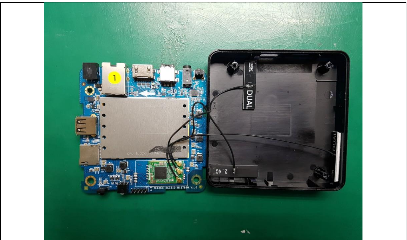
Antenna Connect
