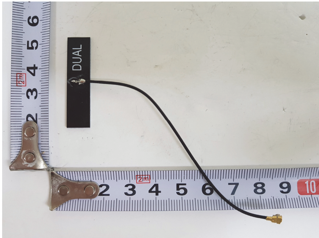
WLAN Antenna 1
