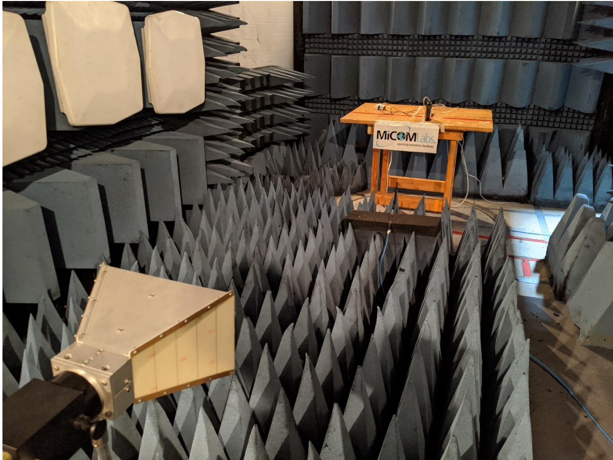
DFS Radiated Test Setup
