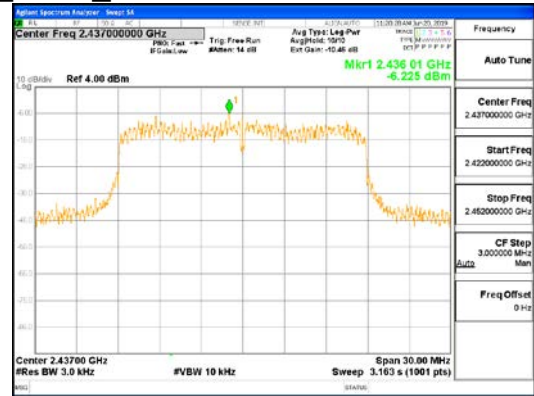
CDD Mode_802.11n_HT20_ANT1
