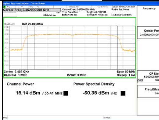
CDD Mode_802.11n_HT40_ANT2
