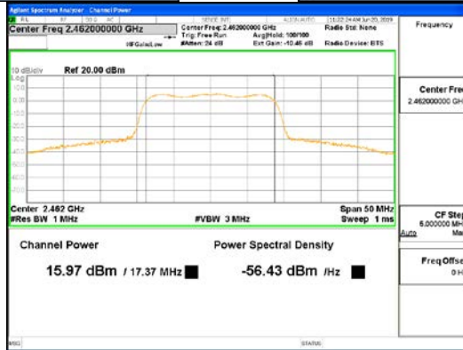
CDD Mode_802.11n_HT20_ANT2
