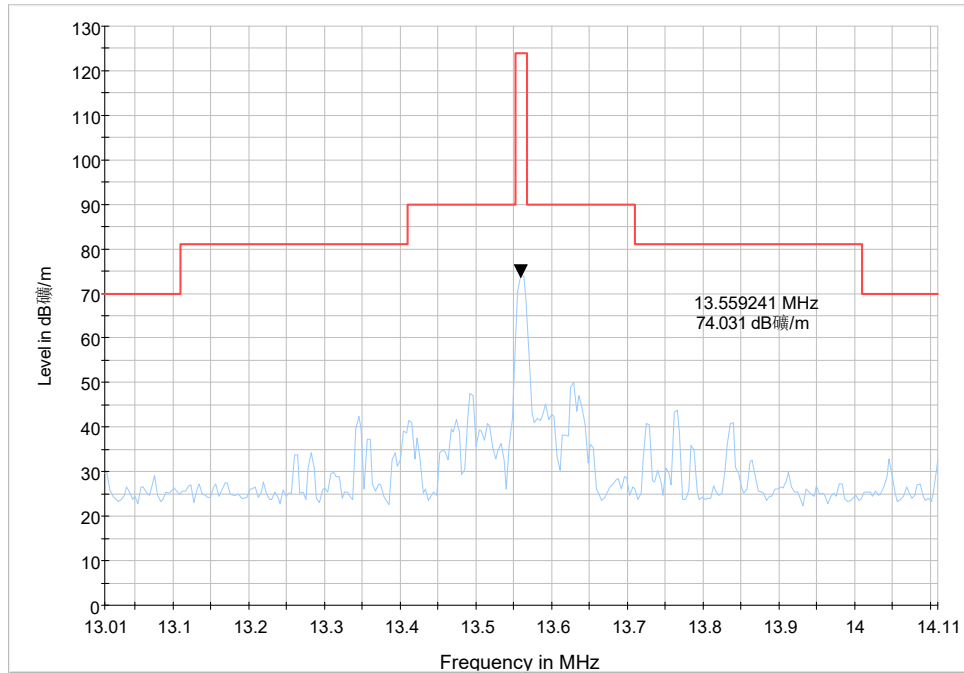
Radiates Emission from 13.01MHz to 14.11MHz
