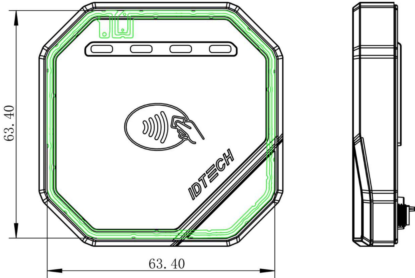
VP7200 contactless NFC antenna
