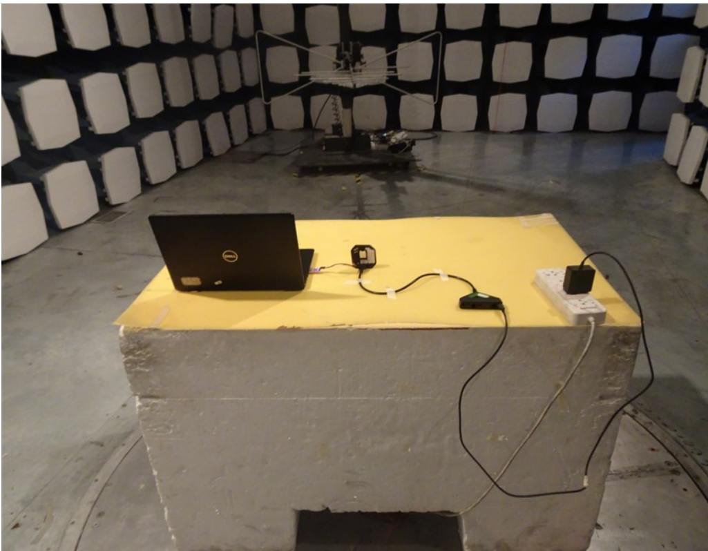
30MHz-1GHz
