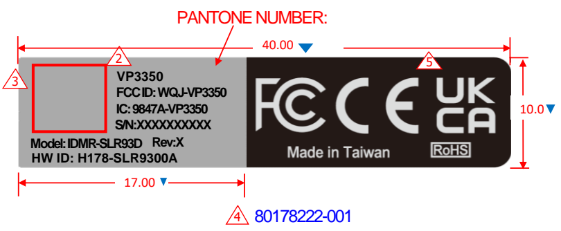
UNIT LABEL PRINTING DETAIL
