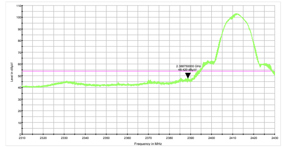
802.11b-Channel 1: Average
