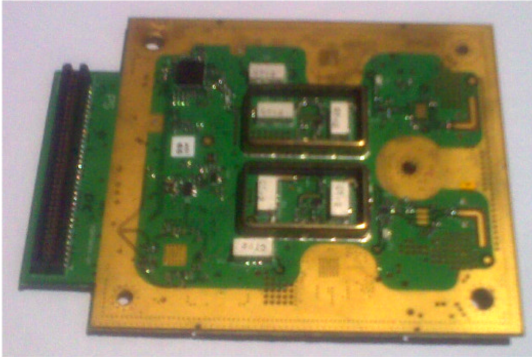
Photograph No.11 RF module second side view without shields
