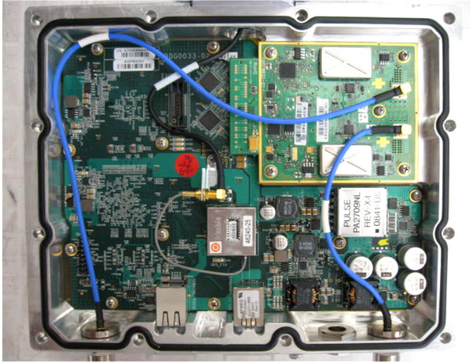
Photograph No.1 Base station WiN7237 internal view
