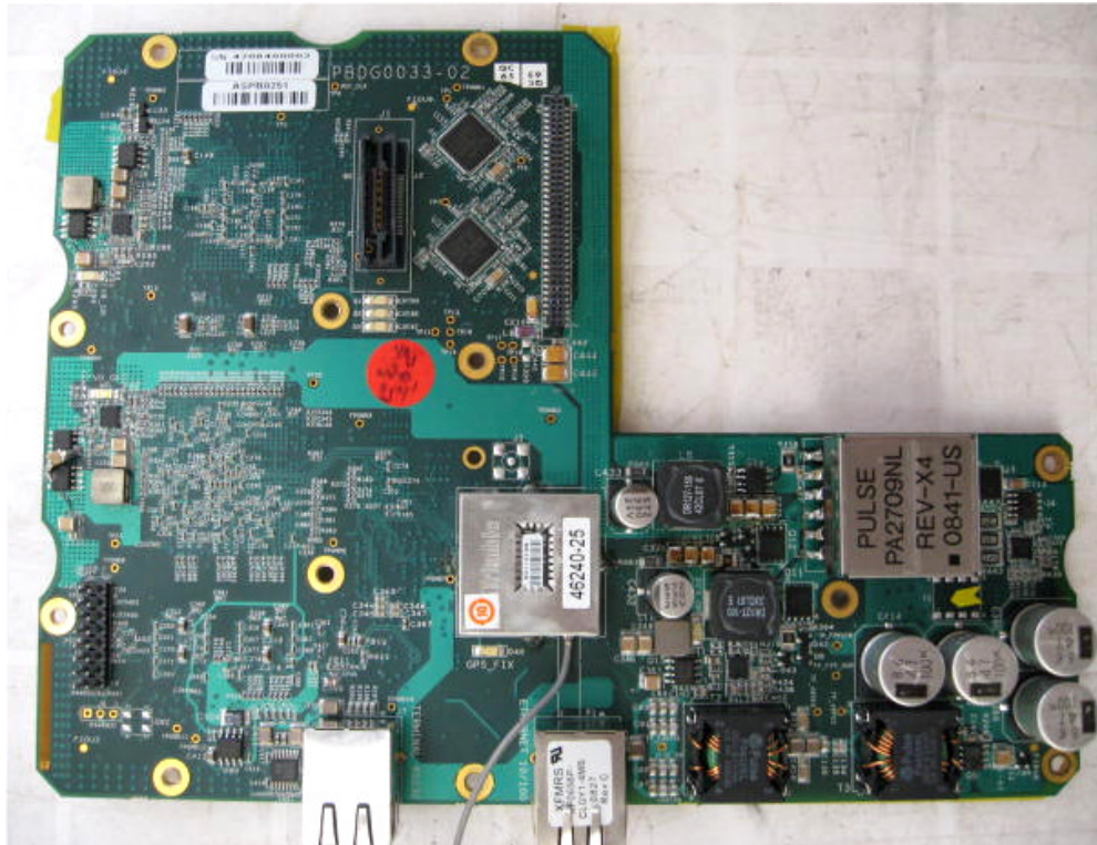
Photograph No.6 Base station WiN7237 main PCB front view
