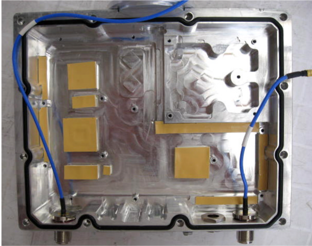
Photograph No.5 Base station WiN7237 chassis
