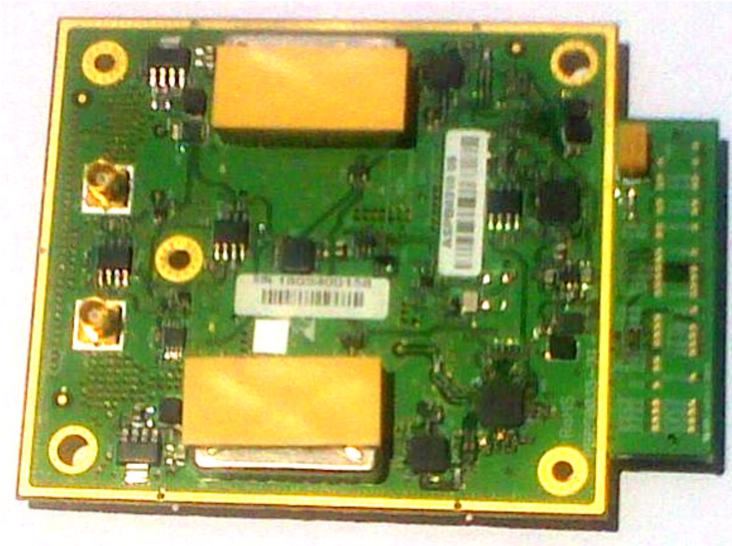
Photograph No.8 RF module front view
