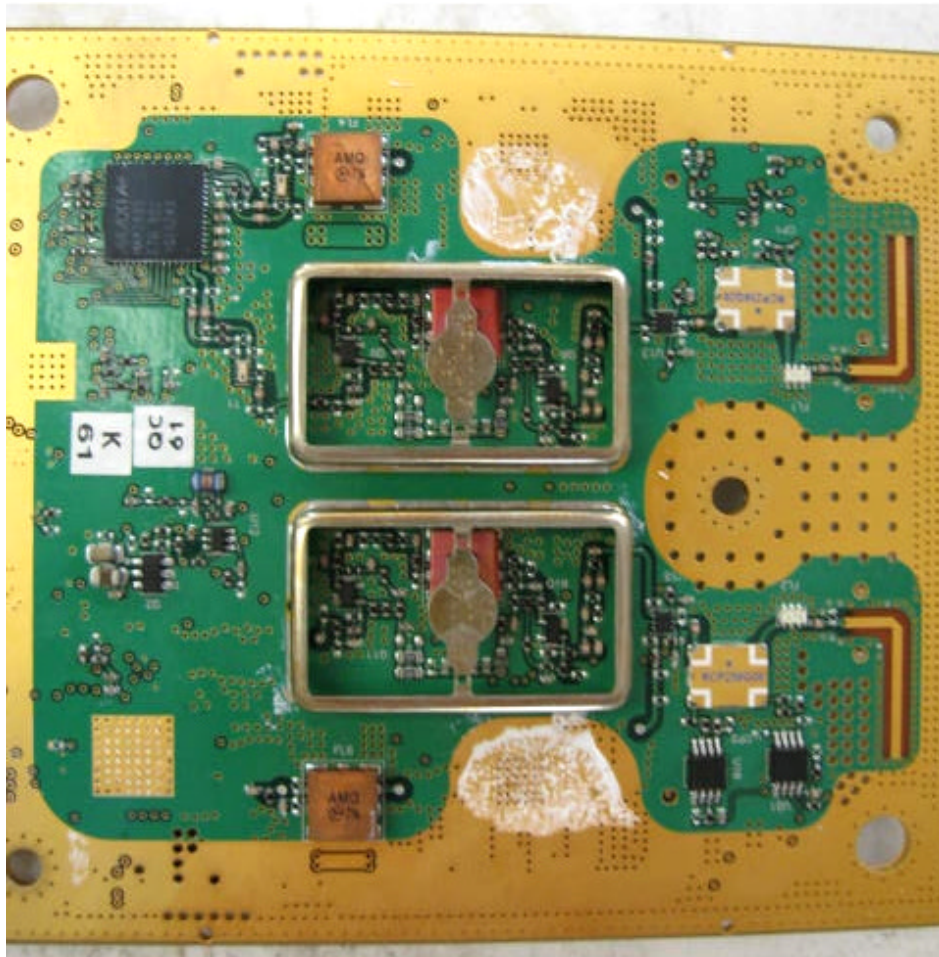
Photograph No.11 RF module second side view without shields
