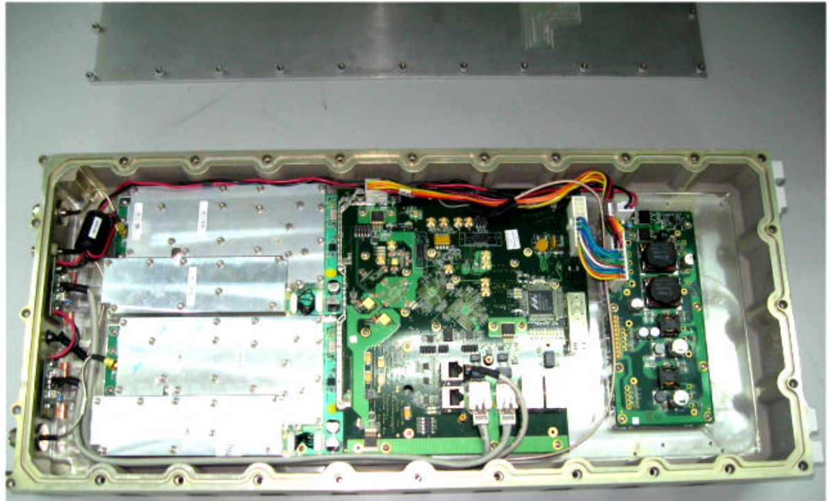
Photograph No.1 Base station WiN7037-2 internal view
