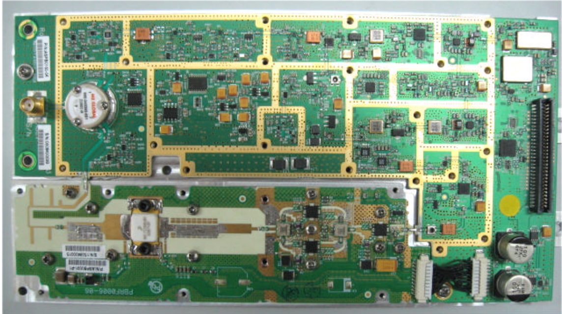
Photograph No.3 WiN7037-2 RF card view without shields
