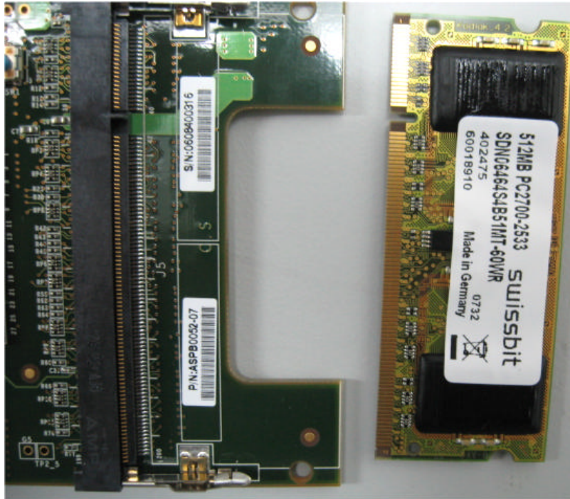
Photograph No.17 Daughter PCB close view
