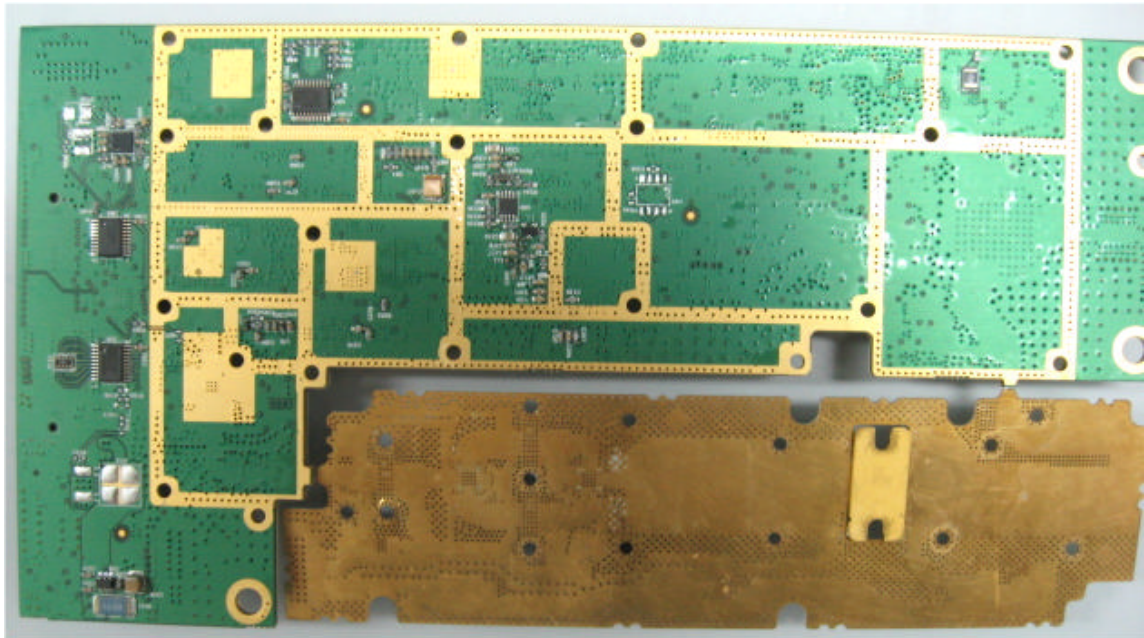
Photograph No.5 WiN7037-2 RF card second side view
