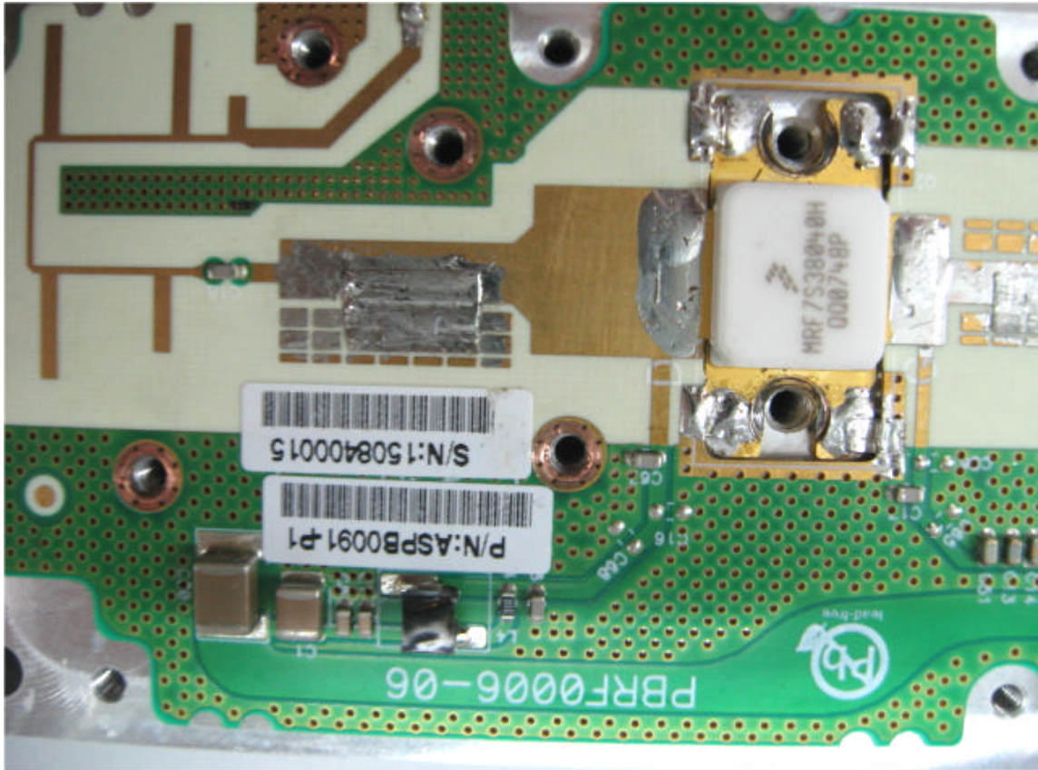
Photograph No.7 WiN7037-2 amplifier card close view
