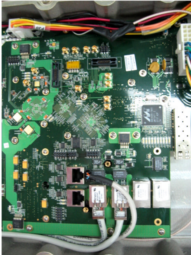
Photograph No.8 WiN7037-2 motherboard view
