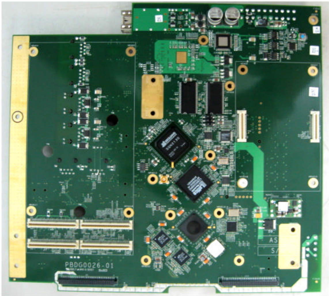
Photograph No.12 WiN7037-2 motherboard without 2 daughter boards
