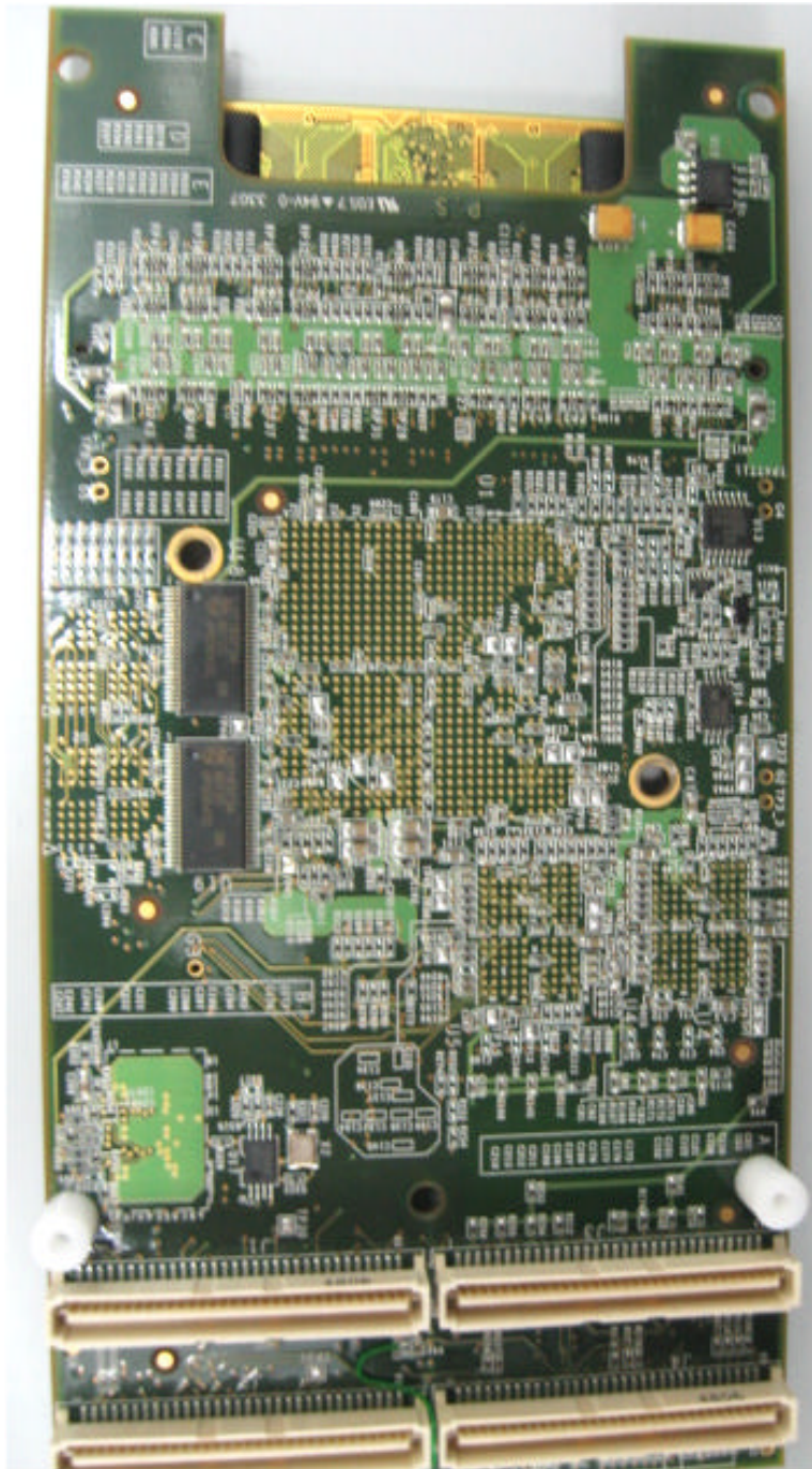
Photograph No.16 Daughter PCB second side view
