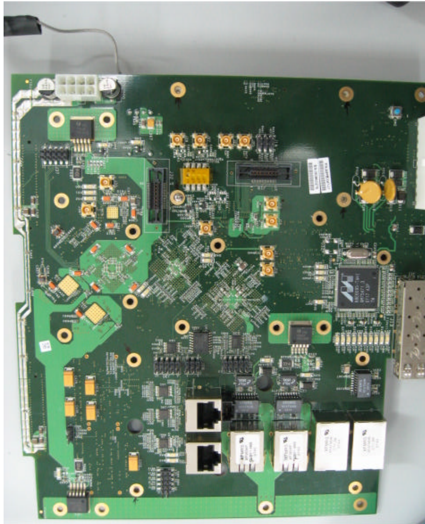
Photograph No.9 WiN7037-2 motherboard without cables view
