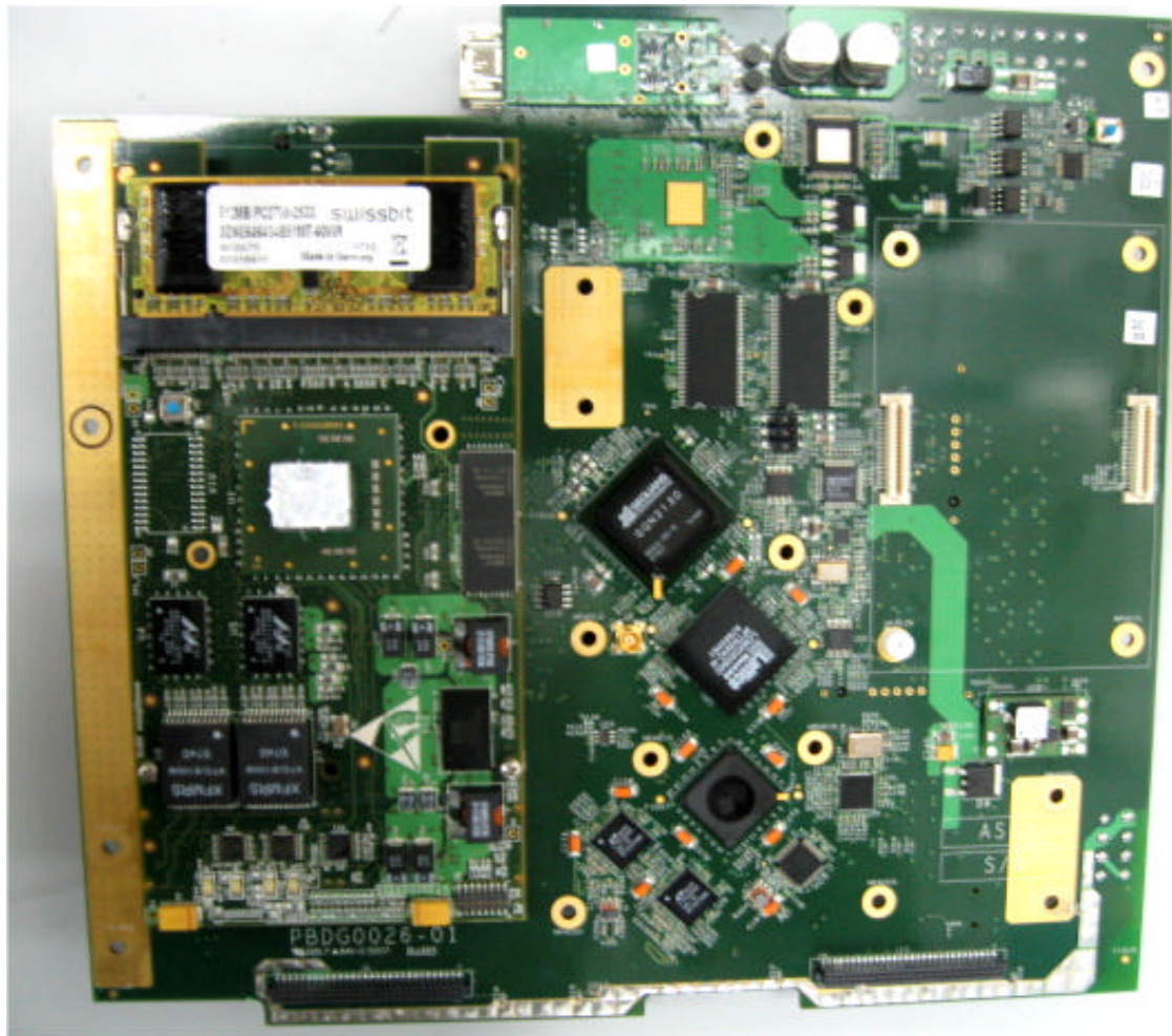
Photograph No.11 WiN7037-2 motherboard second side with daughter board
