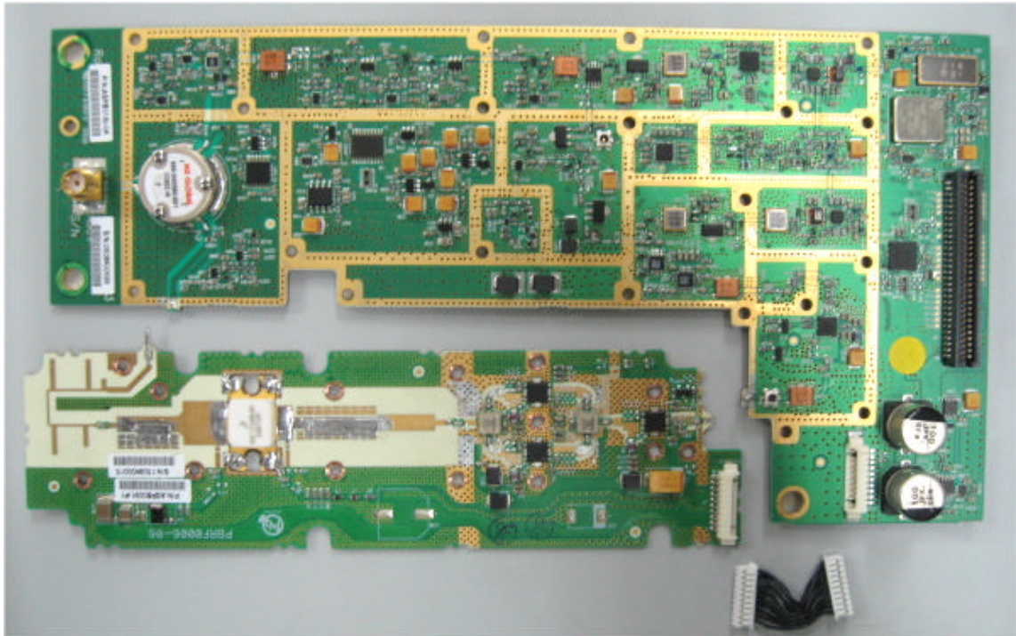
Photograph No.4 WiN7037-2 RF card with amplifier removed
