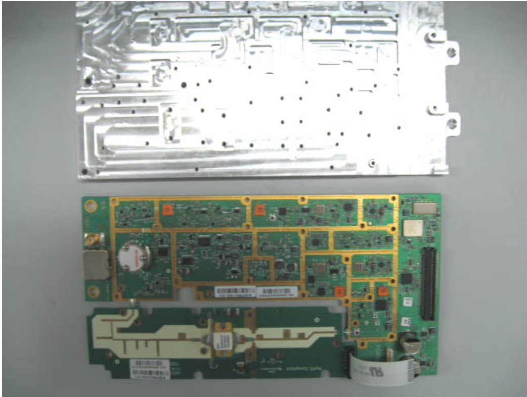
Photograph No.14 RF module front view with shield removed
