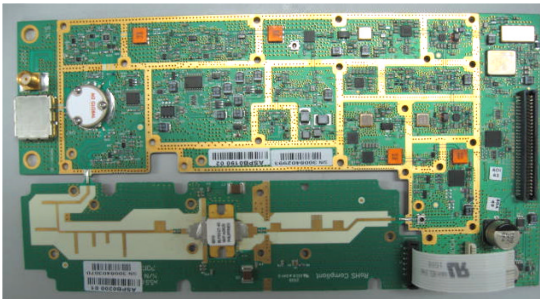
Photograph No.15 RF module PCB front view
