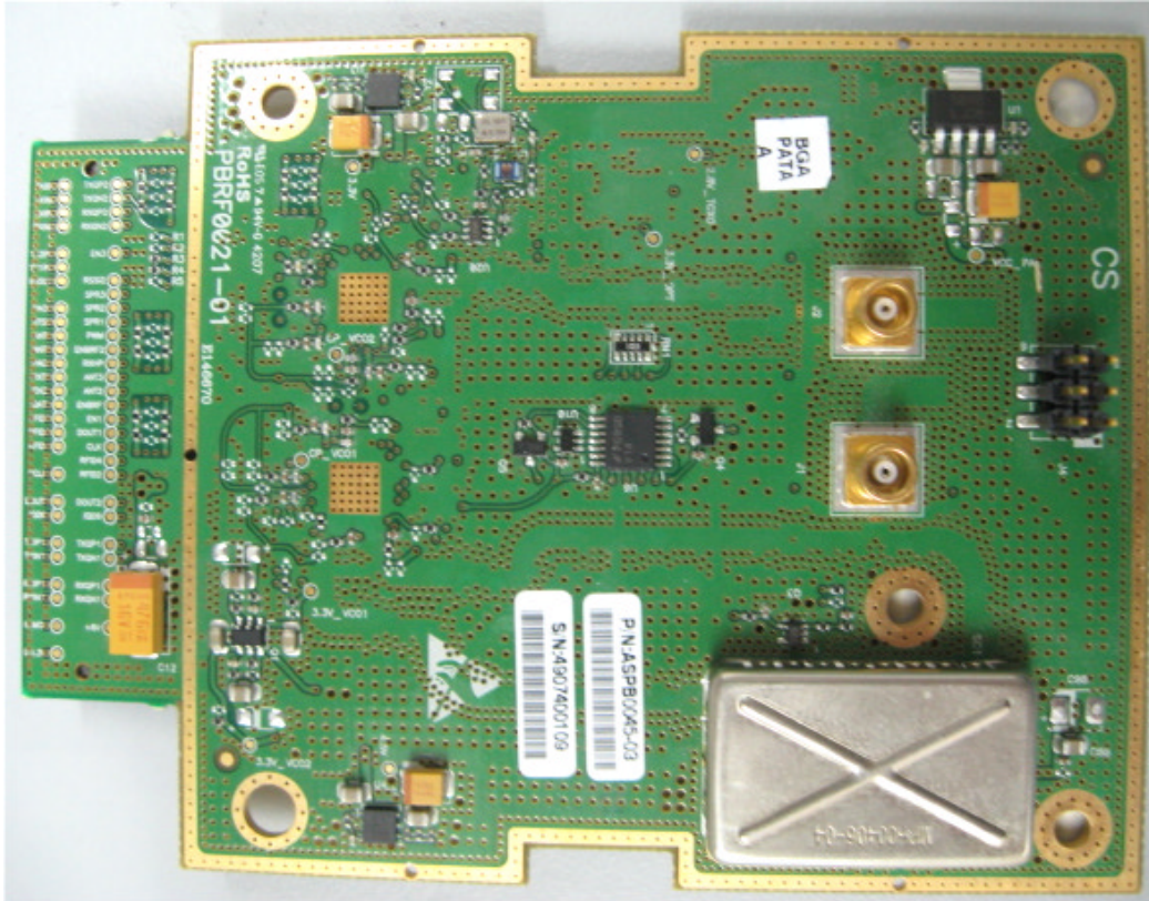
Photograph No.5 Subscriber unit RF card front view
