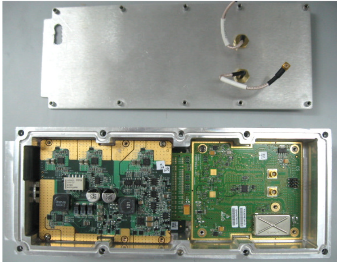
Photograph No.1 Subscriber unit WiN5235 internal view
