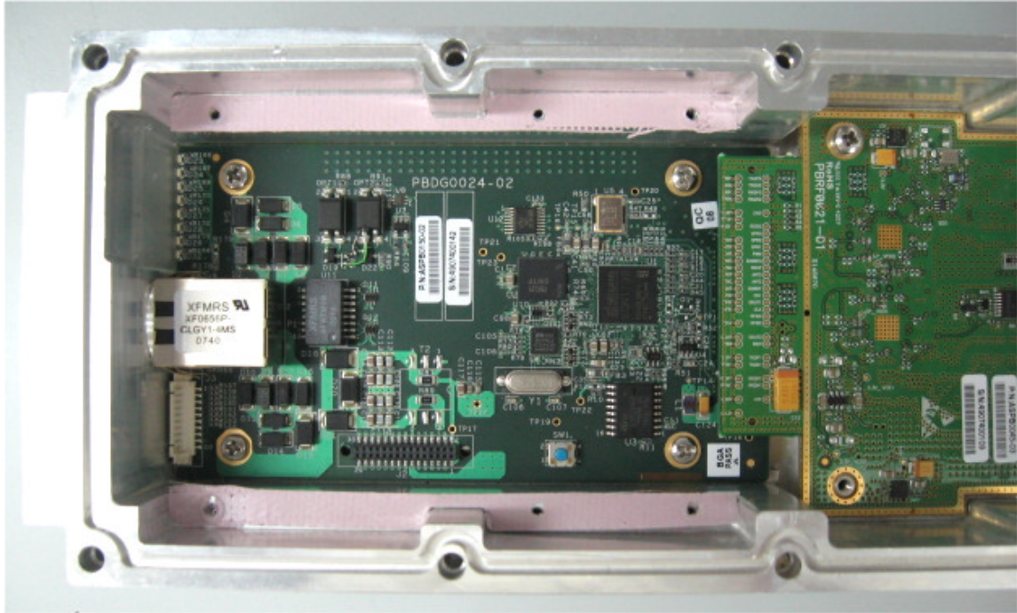
Photograph No.4 Subscriber unit Win5235 internal view with PA PCB removed
