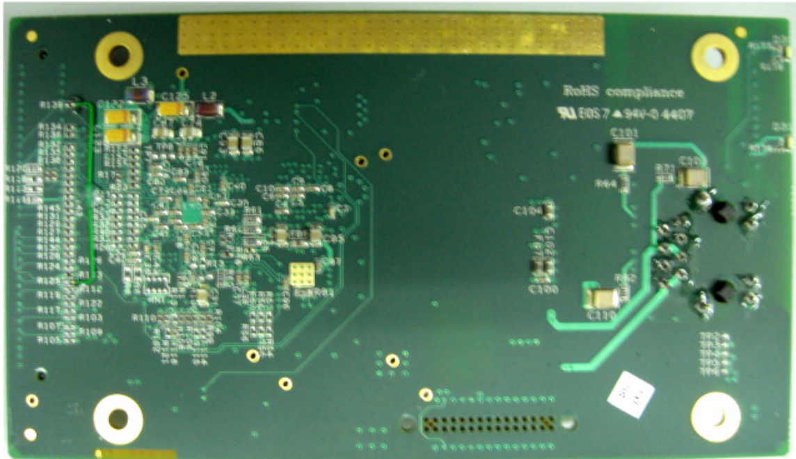
Photograph No.9 Subscriber unit main PCB second side view
