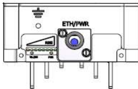
Figure 2-5: Interconnection Panel
