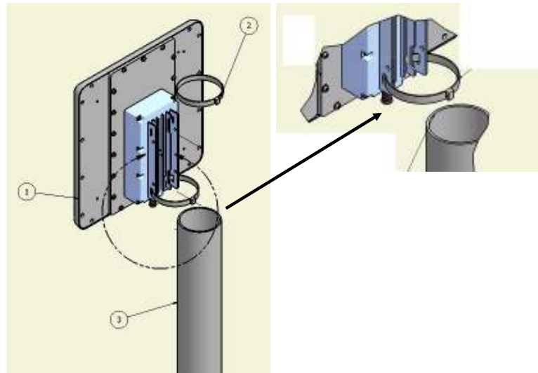
Figure 4-1: Pole Mounting
