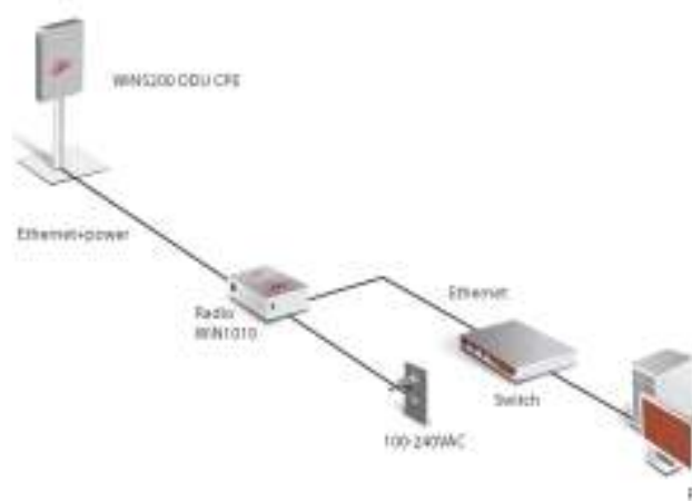
Figure 4-4: WiN5200 Interconnection Schema
