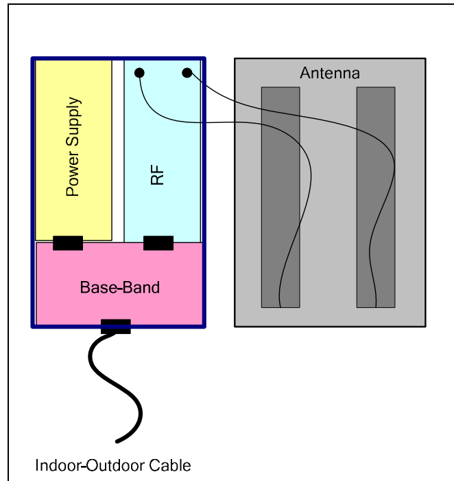
Figure 2-2: WiN5200 Block Diagram
