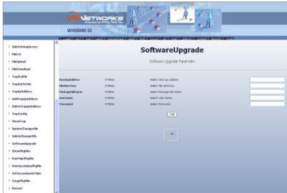
Figure 6-1: SoftwareUpgrade Screen
