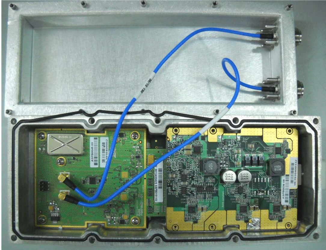
Photograph No.1 Subscriber unit WiN5137 internal view
