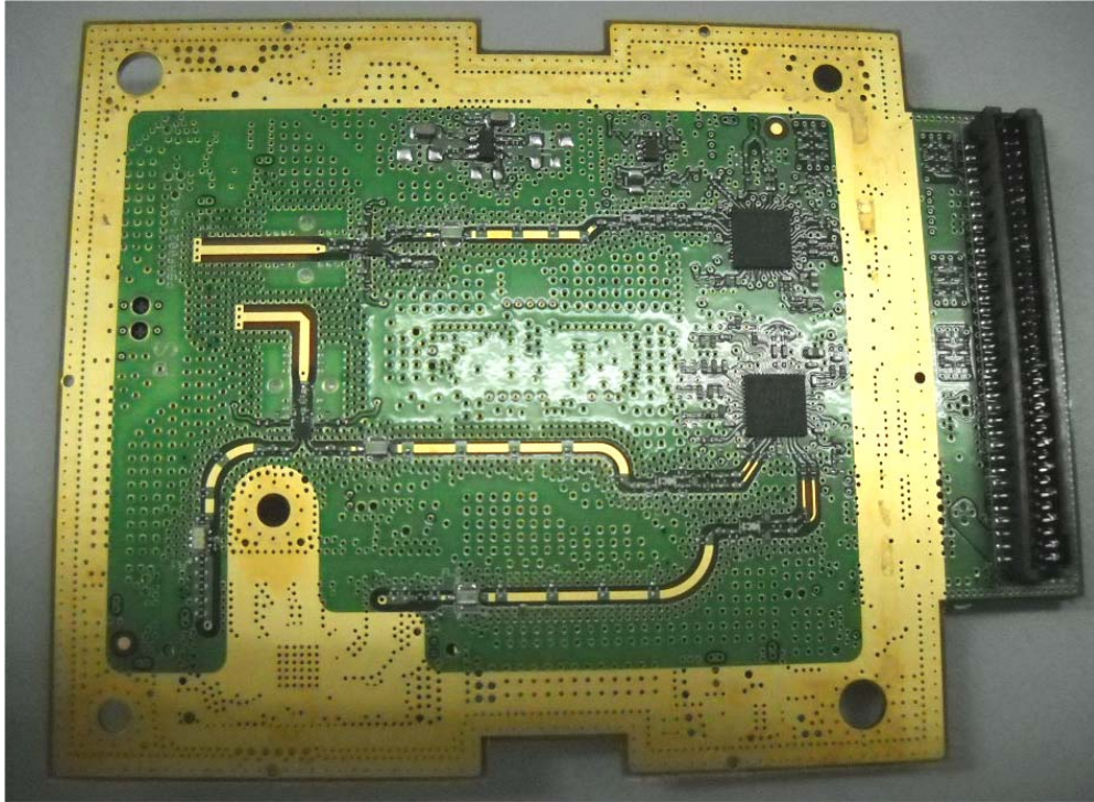
Photograph No.6 Subscriber unit RF card second side view
