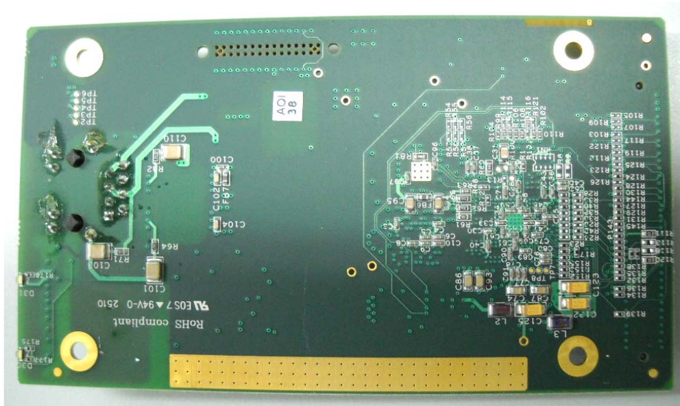
Photograph No.9 Subscriber unit main PCB second side view
