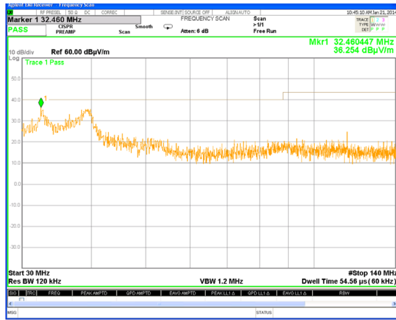
Plot # 5. Pre compliance frequencies scan from 30 to 140 MHz. Test distance 3m.
