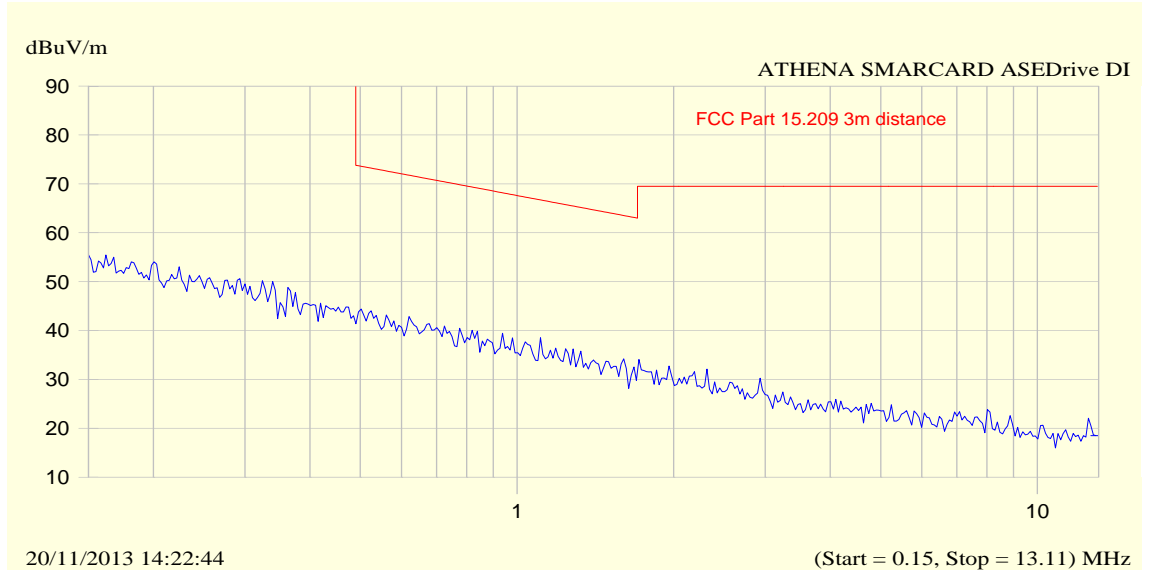
Plot # 3. Frequencies scan 0.15 – 13.11 MHz. Test distance =3m.
