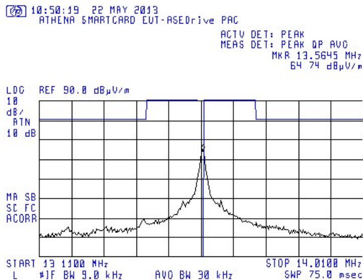
Plot # 2. Frequencies scan 13.11 – 14.01 MHz. Test distance =3m.
