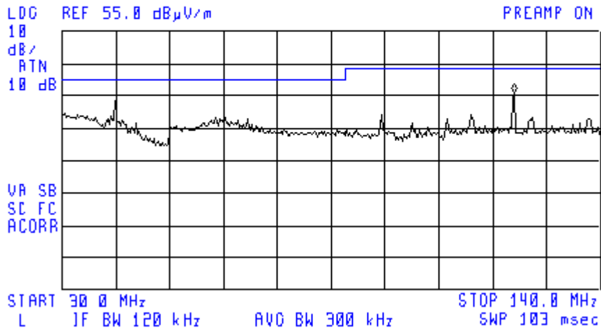
Plot # 5. Frequencies scan 30 – 140 MHz. Test distance 3m.
