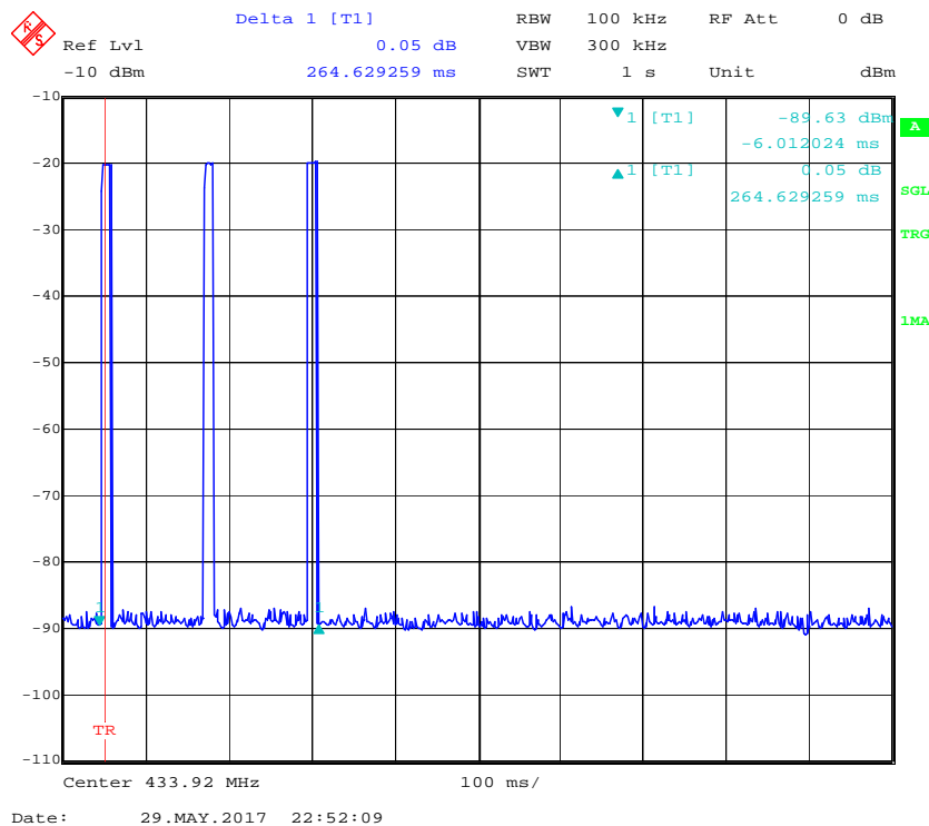
Transmission period
