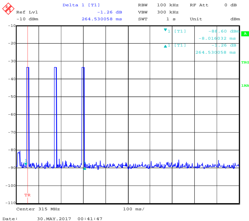
Transmission period
