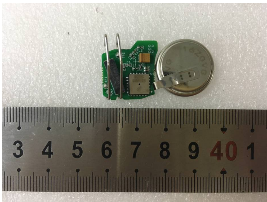
EUT –Battery &Main Board Front View
