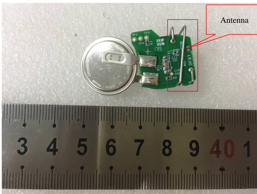
EUT –Battery &Main Board RearView
