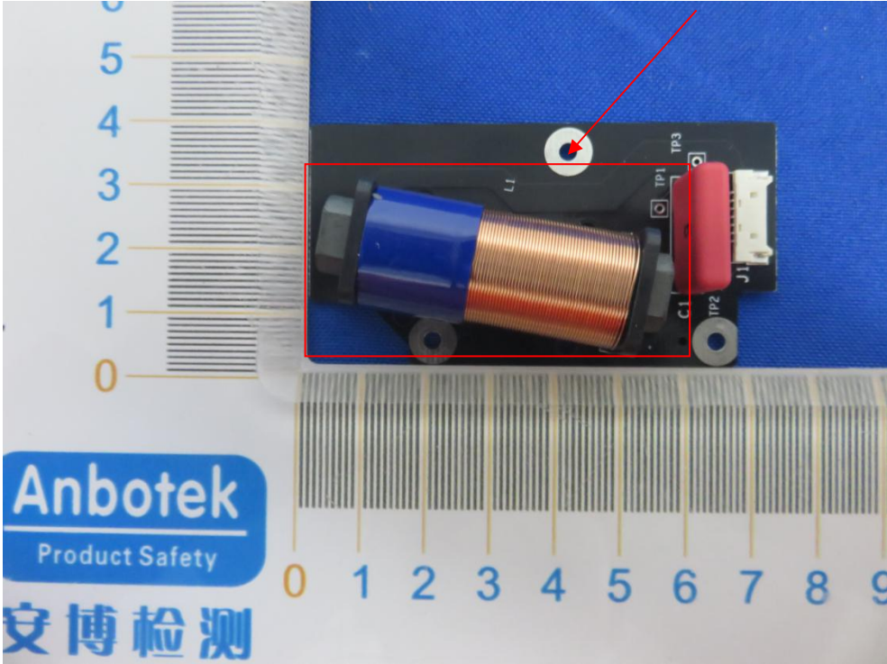
125KHz Antenna
