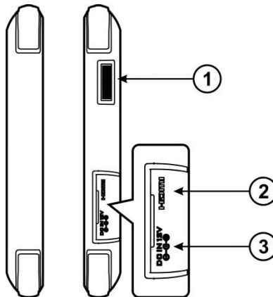
Figure 2-3 MaxiSys Tablet Left Side
