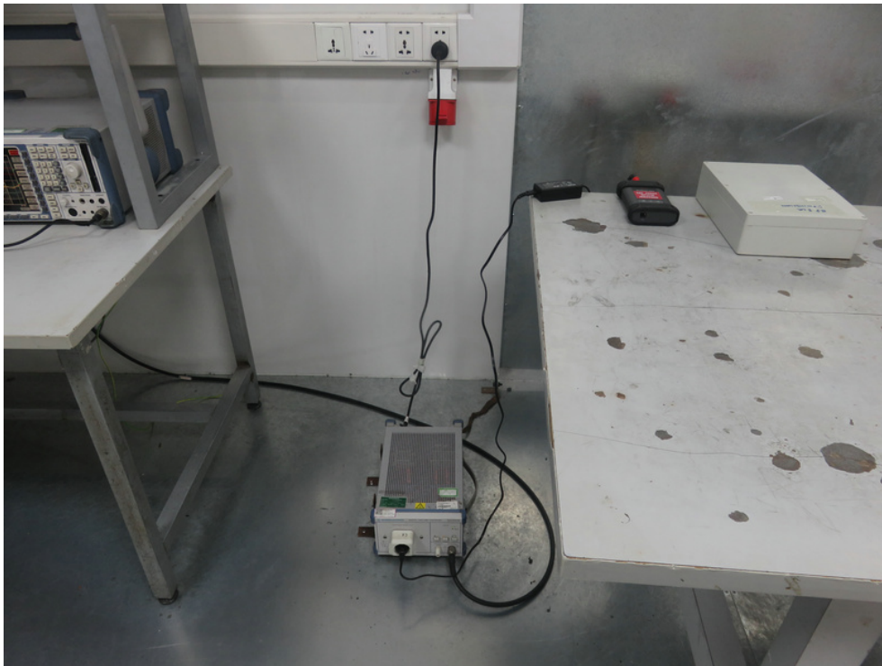
FCC ID: WQ8MAXIFLASHULTRA Photo of Conducted Emission Measurement
