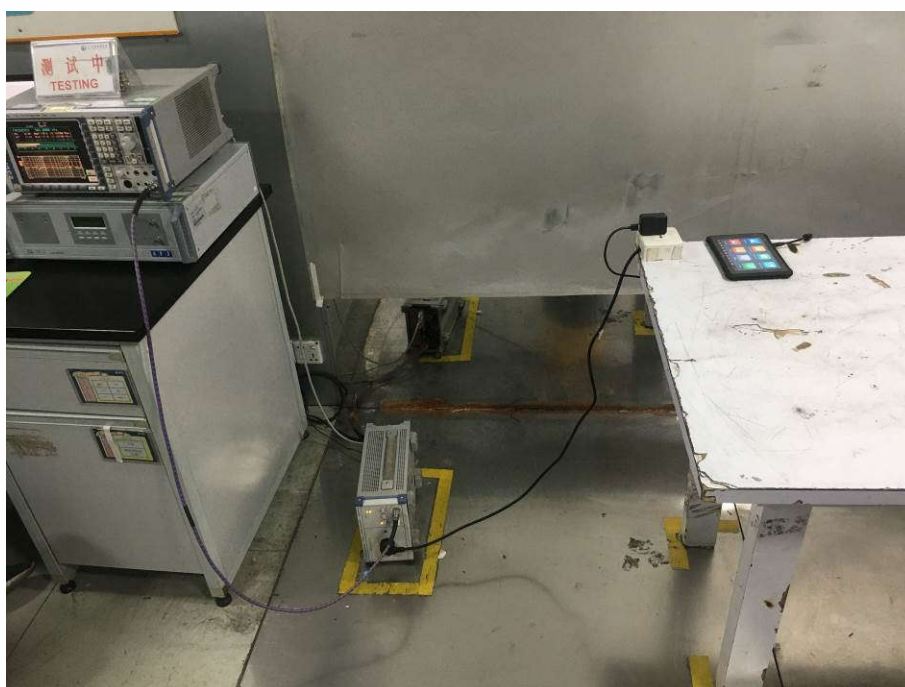
Radiated spurious emission Test Setup-4(CE)
