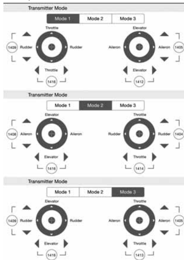
Figure 4-18 Mode 1, 2 and 3
