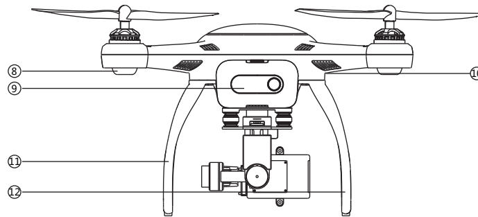
Figure 2-2 Rear Side
