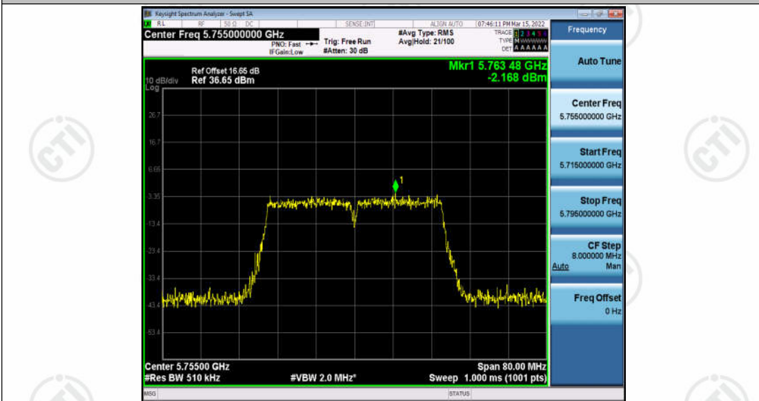
11AC40SISO_Ant2_5755
