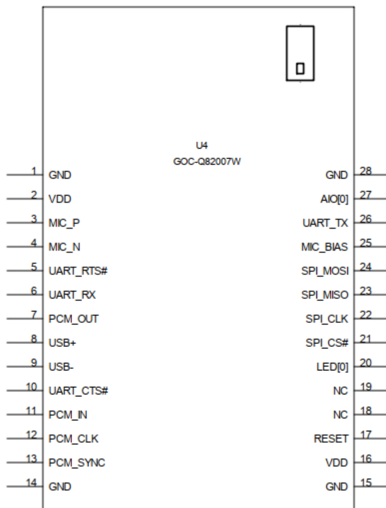
Figure 2: Pin Diagram
