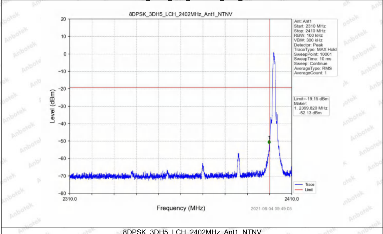
8DPSK_3DH5_LCH_2402MHz_Ant1_NTNV
