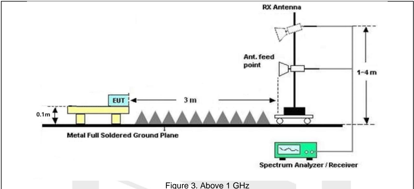
Figure 3. Above 1 GHz
