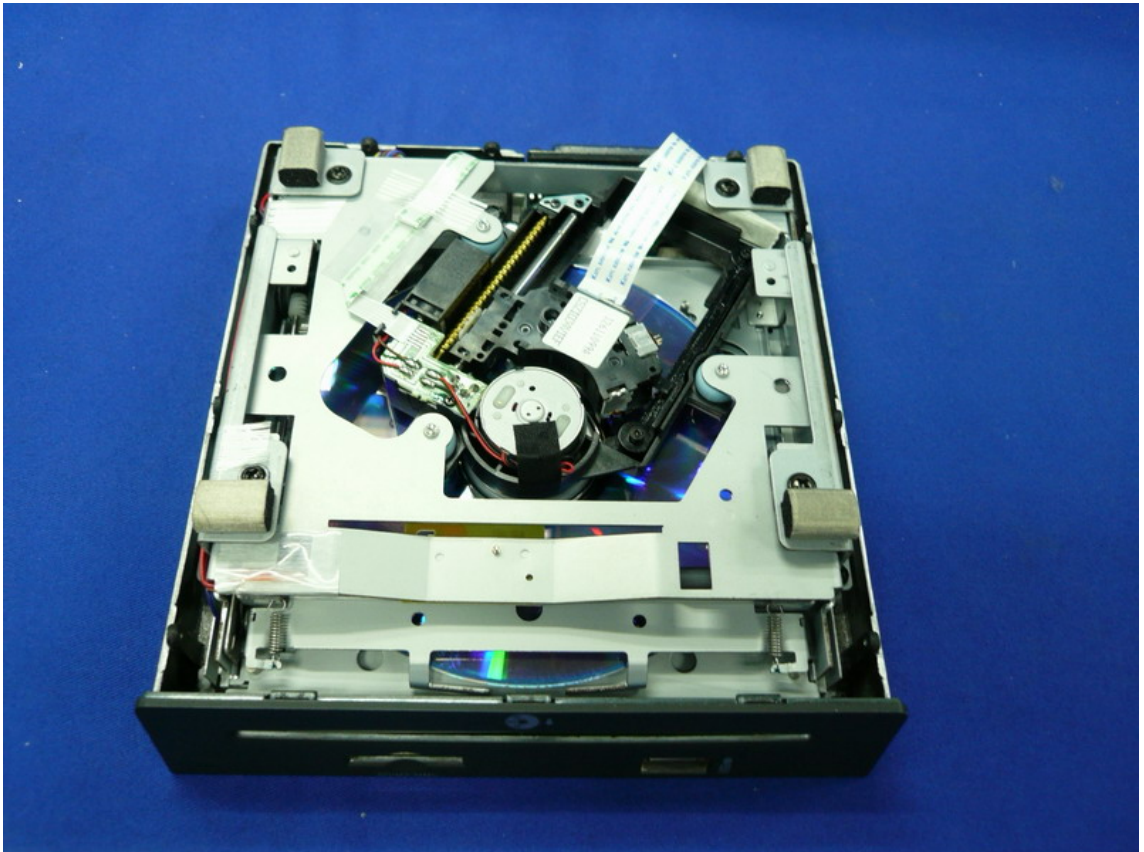
Figure 35 Inside of the External functional module
