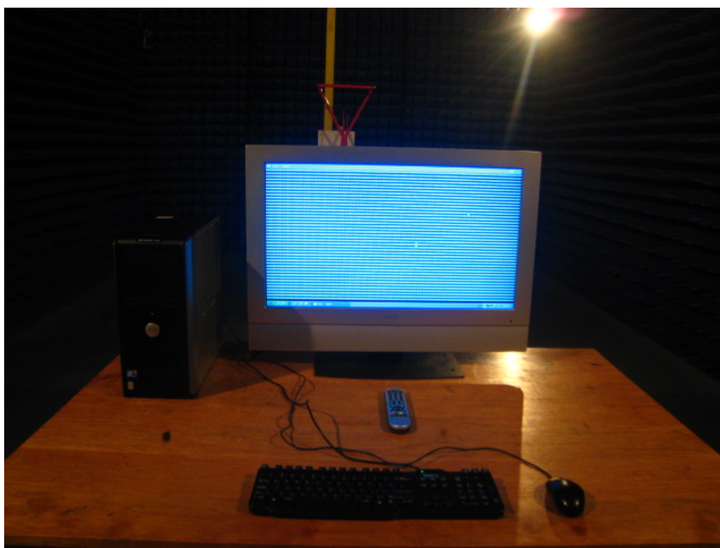
Test photo of radiated emission (30MHz-1000MHz)
