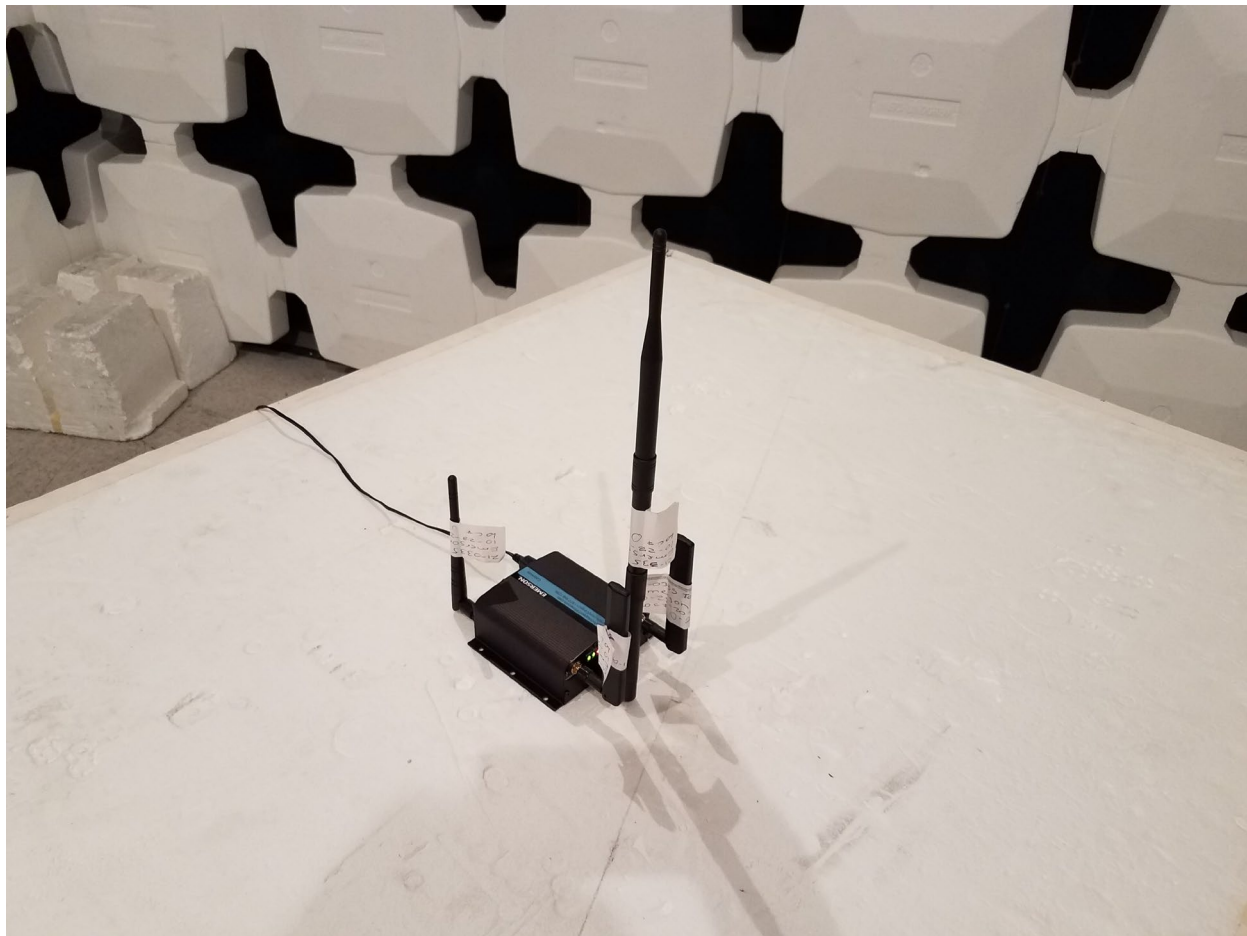
Figure 1. EUT Test Configuration for Unwanted Spurious Emissions
