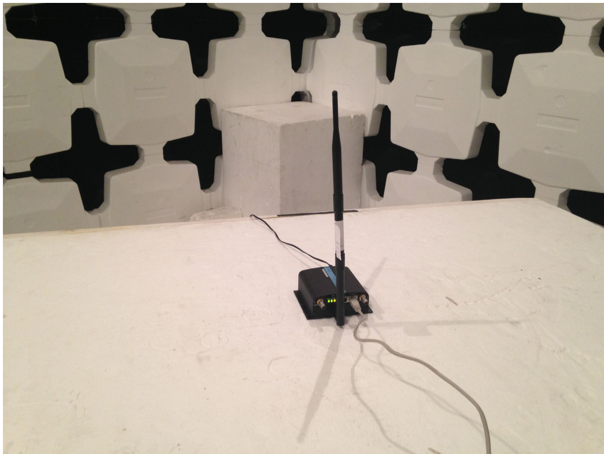
Figure 2. EUT Test Configuration for Intentional Emissions
