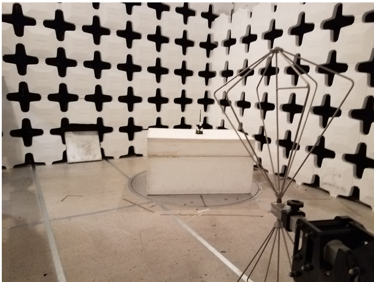
Figure 3. Radiated Emissions, 30-200 MHz
