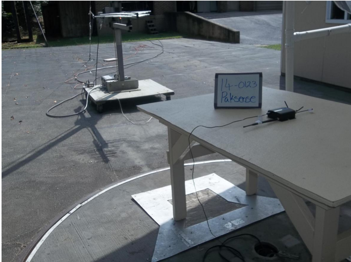
Photo 6- Fundamental Emissions Test Setup, without RF Label, Back
