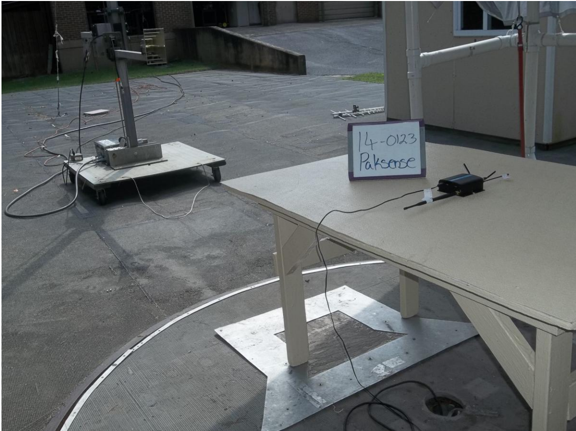
Photo- 8 Harmonics Measurement, without RF Label, Back
